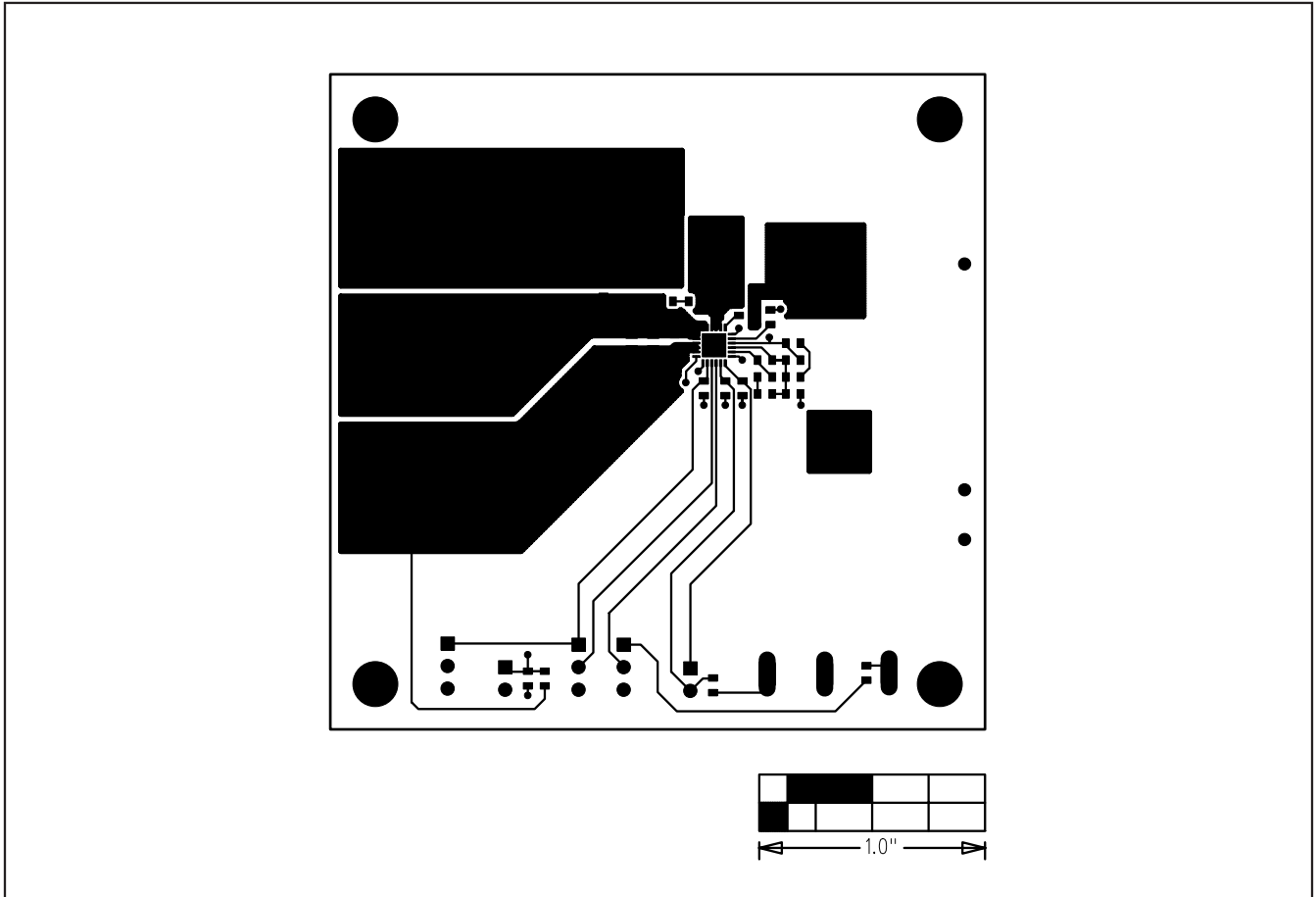
Figure 3. MAX15039 EV Kit PCB Layout—Component Side
