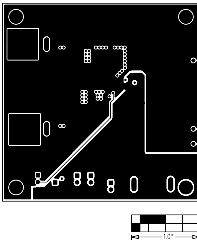
Figure 4. MAX15039 EV Kit PCB Layout—Layer 2
