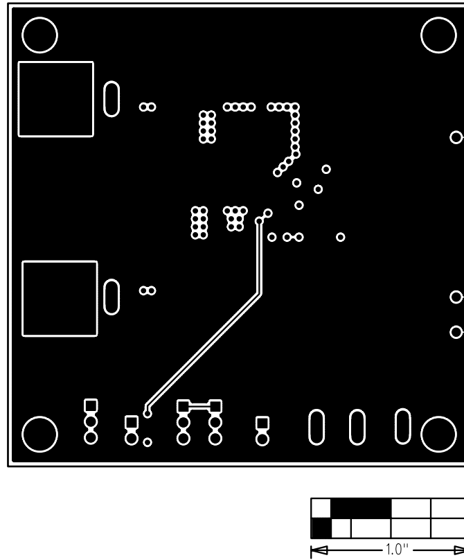
Figure 5. MAX15039 EV Kit PCB Layout—Layer 3
