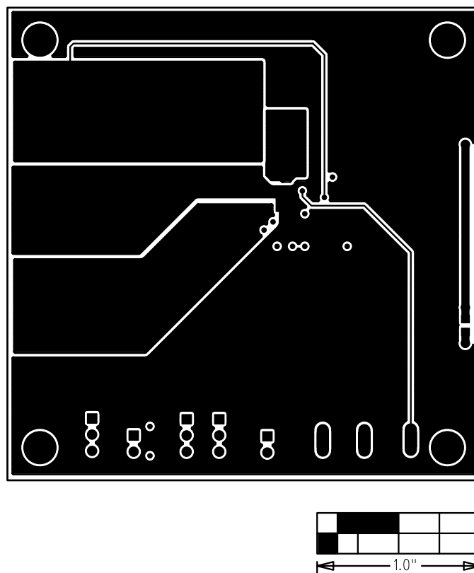
Figure 6. MAX15039 EV Kit PCB Layout—Solder Side
