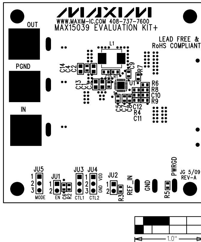
Figure 2. MAX15039 EV Kit Component Placement Guide—Component Side
