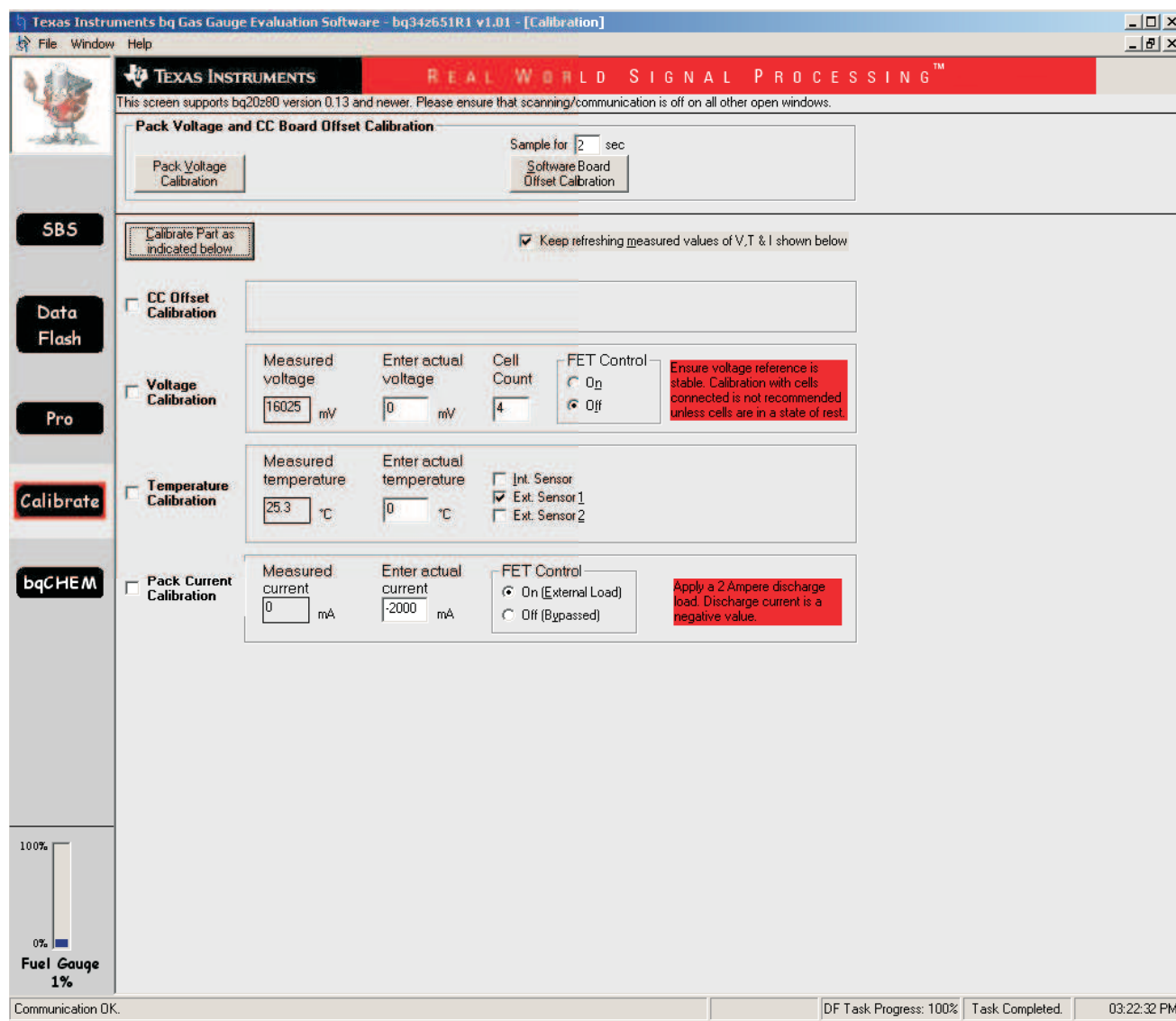
Figure 10. Calibration Screen
