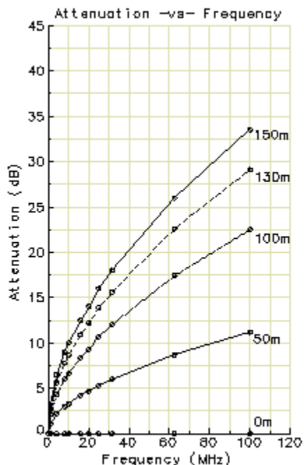
Figure 3-10 EIA/TIA Attenuation vs. Frequency for 0, 50, 100, 130 & 150 meters of CAT 5 cable
