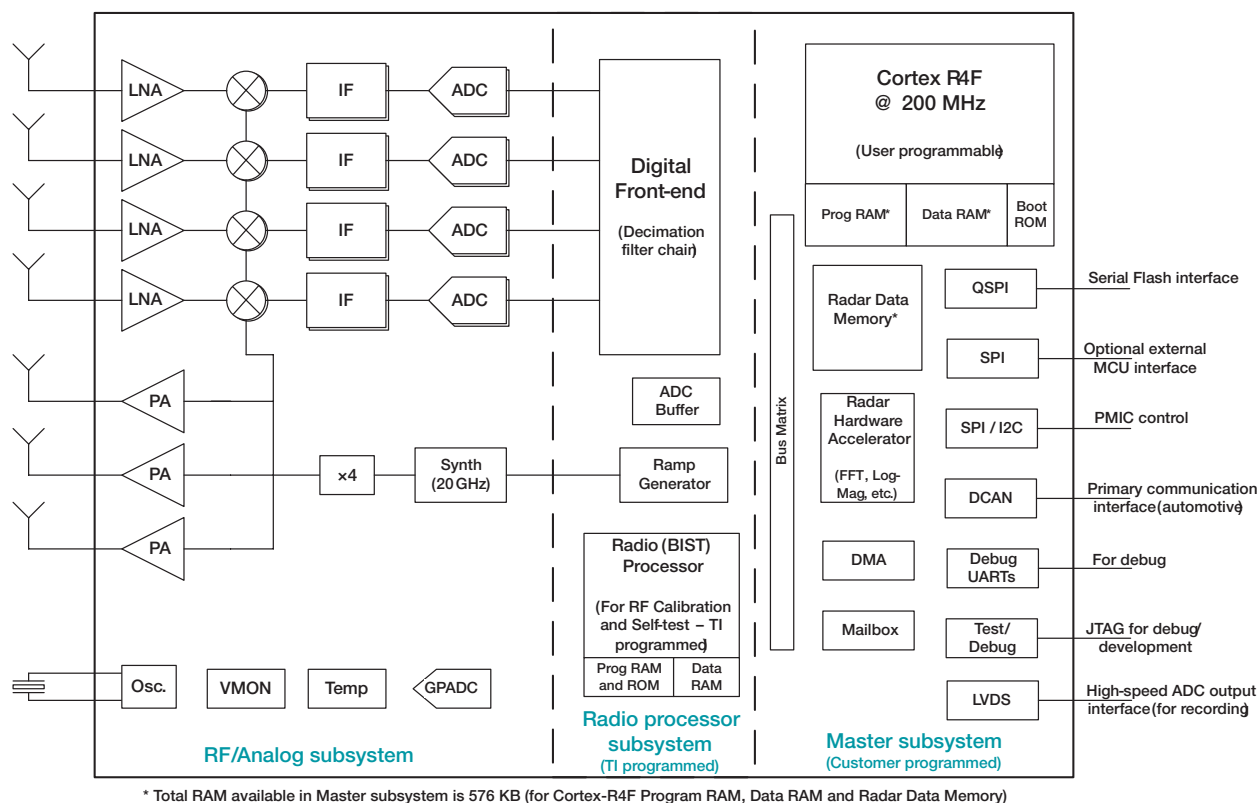
Figure 1. AWR1443 radar high-level architecture.
