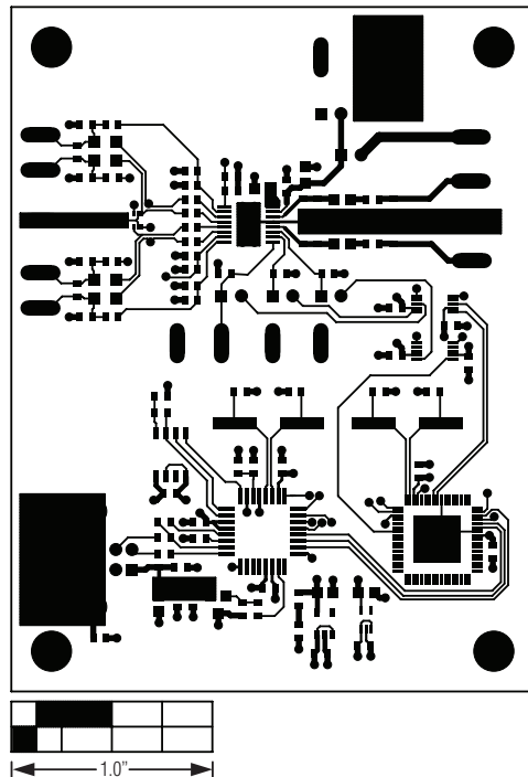
Figure 5. MAX13335E EV Kit PCB Layout—Component Side
