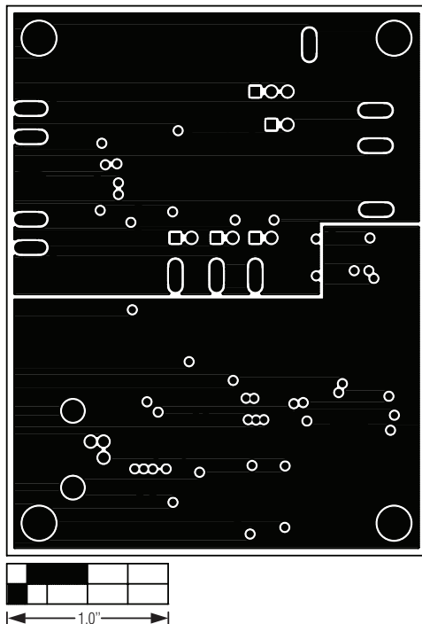
Figure 6. MAX1335E EV Kit PCB Layout—GND Layer 2
