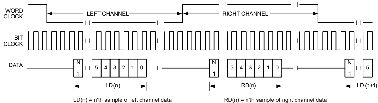
Figure 5-40. Timing Diagram for I²S Mode With Offset = 2
