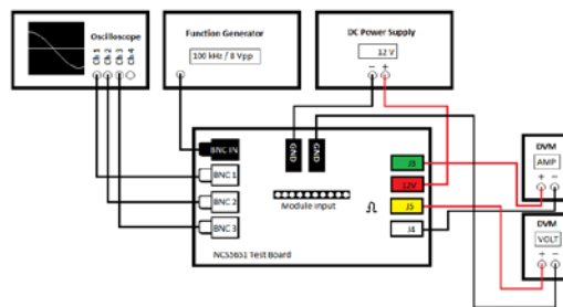
Figure 1: Testboard NCS5651
