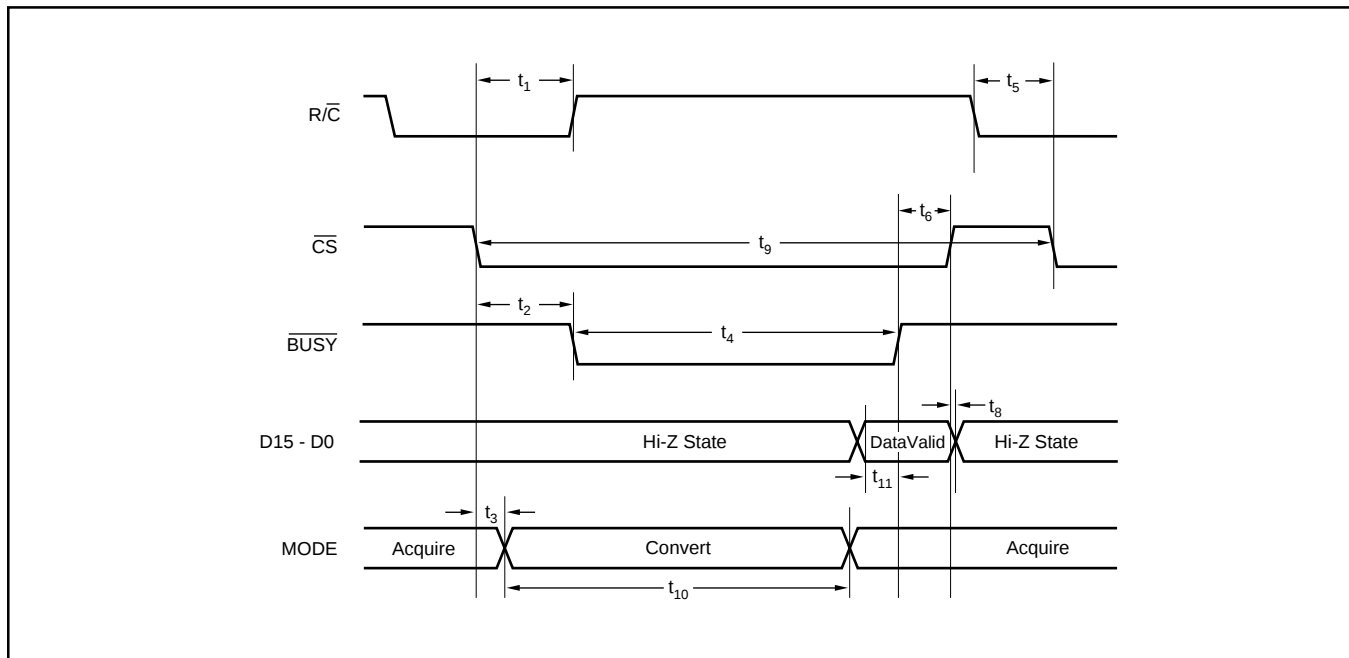
FIGURE 2. ADS7815 Timing.
