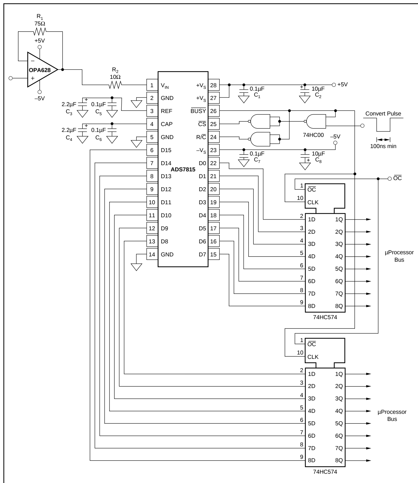
FIGURE 1. Basic Operation.
