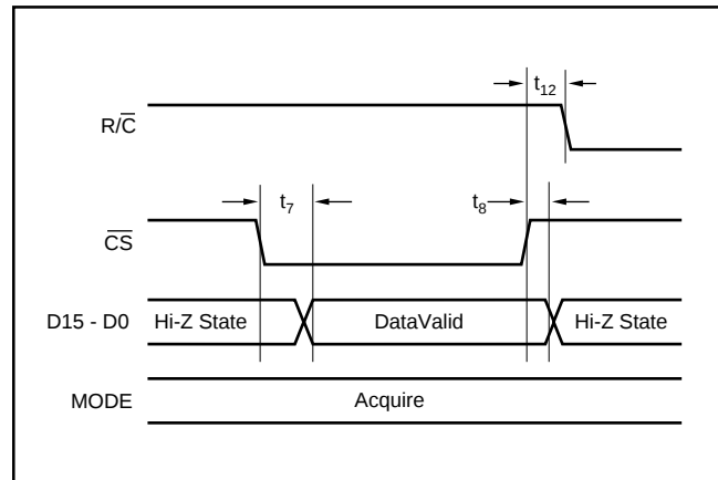
FIGURE 3. Bus Timing.
