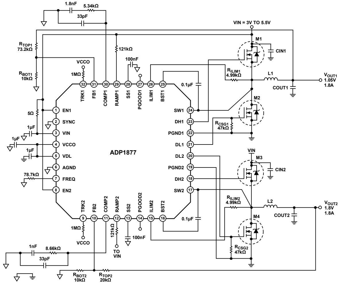
Figure 44. Typical Low Current Application with V_{IN} < 5.5\text{V}
