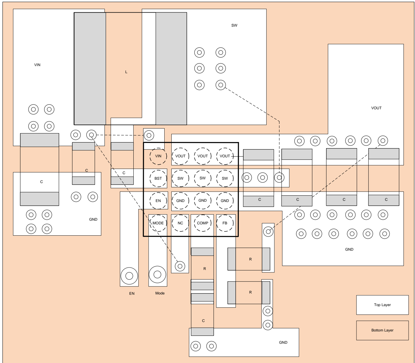
Figure 18. Recommended Layout
