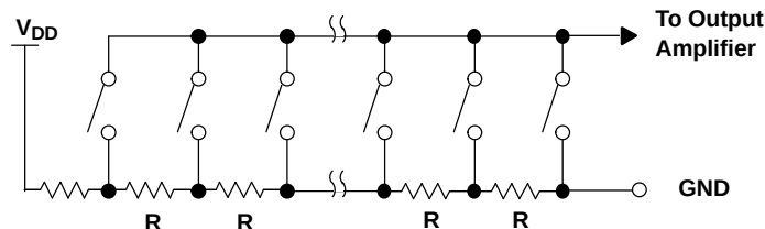
Figure 40. Resistor String
