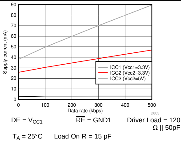
Figure 5. ISO141x Supply Current Vs Data Rate- With 120\Omega||50\text{pF} Load
