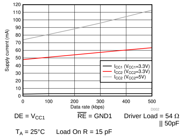
Figure 4. ISO141x Supply Current Vs Data Rate- With 54\Omega||50\text{pF} Load
