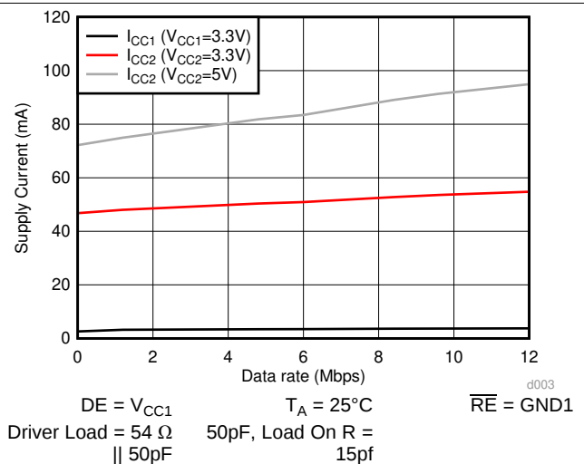
Figure 8. ISO143x Supply Current Vs Data Rate- 54\Omega||50\text{pF} Load
