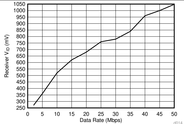
Figure 28. ISO145x Receiver V_{ID} vs Signaling Rate
