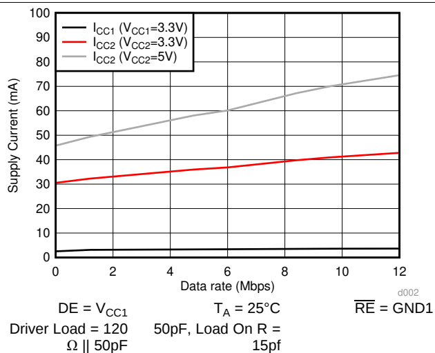
Figure 5. ISO141x Supply Current Vs Data Rate- With 120\Omega||50\text{pF} Load
