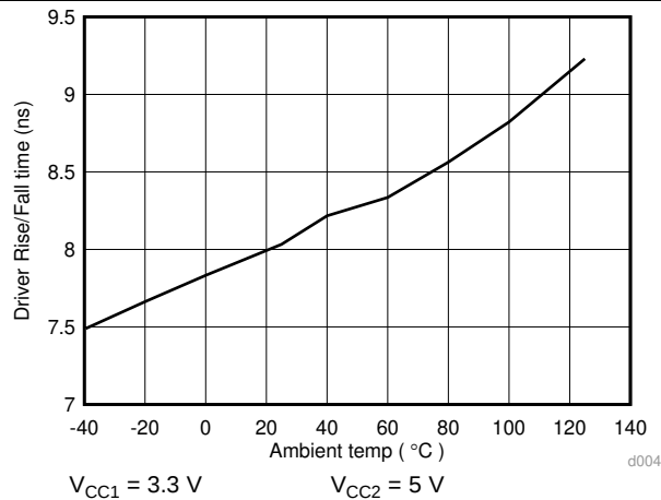
Figure 17. ISO143x Driver Rise/Fall Time (ns) Vs Temperature ( ^\circ C )
