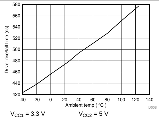
Figure 16. ISO141x Driver Rise/fall Time (ns) Vs Temperature ( ^\circ C )
