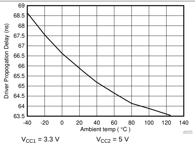
Figure 20. ISO143x Driver Propagation Delay (ns) Vs Temperature ( ^\circ C )
