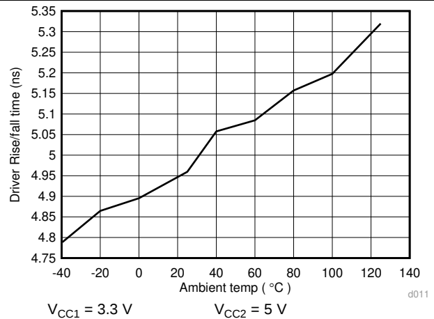
Figure 18. ISO145x Driver Rise/Fall Time (ns) Vs Temperature ( ^\circ C )
