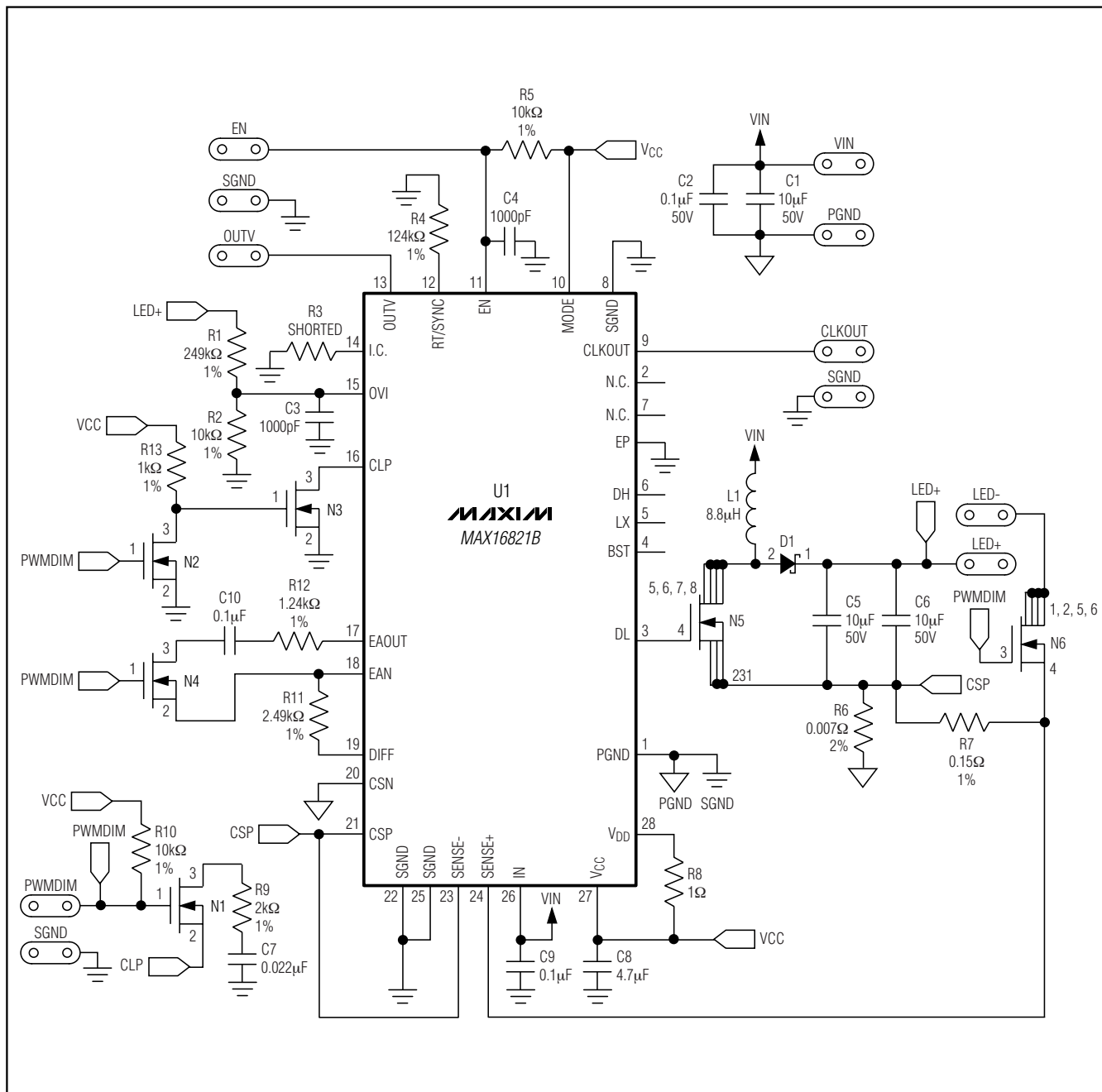
Figure 1. MAX16821B EV Kit Schematic
