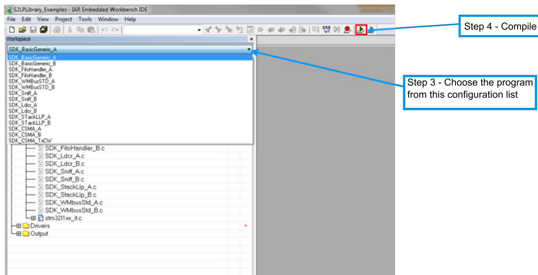
Figure 29. IAR project
