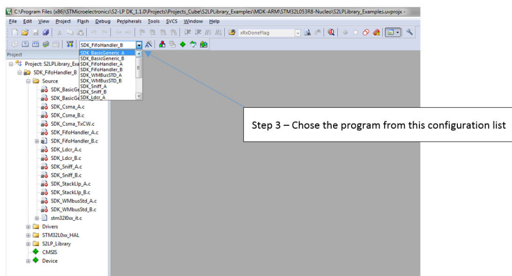
Figure 30. Keil project
