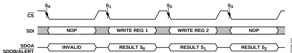
Figure 46. Register Write
