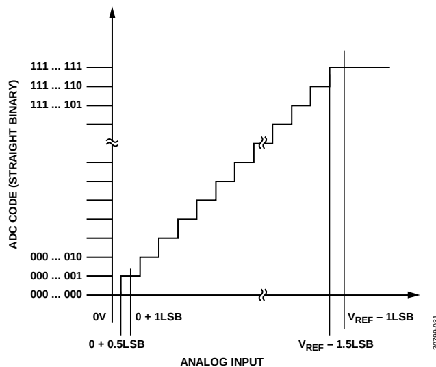
Figure 29. ADC Ideal Transfer Function
