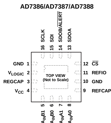
Figure 7. Pin Configuration
