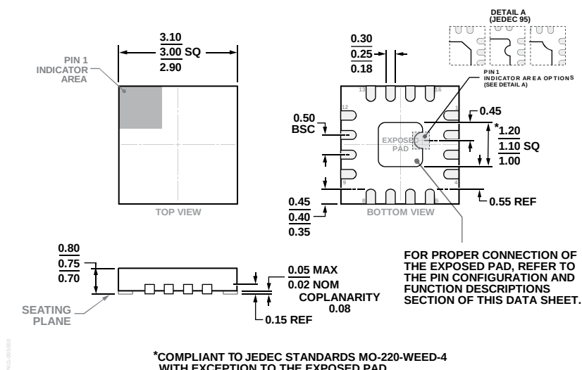
Figure 48. 16-Lead Lead Frame Chip Scale Package [LFCSP] 3 mm x 3 mm Body and 0.75 mm Package Height (CP-16-45)
