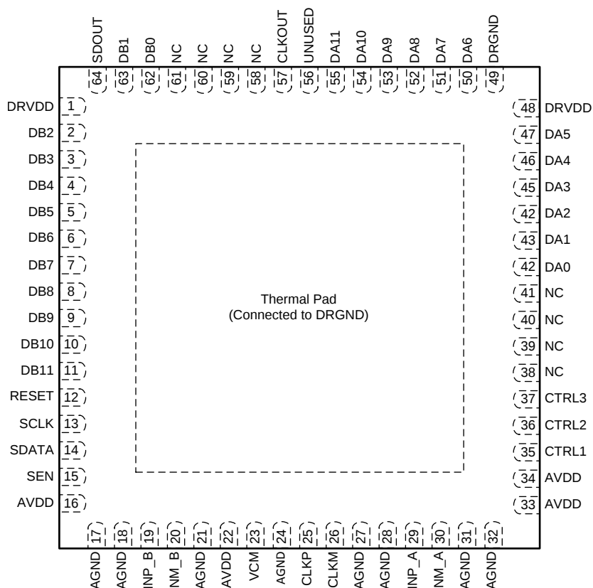
Pin Functions – CMOS Mode
