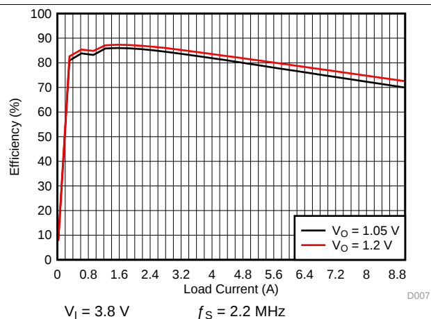
Figure 5-7. SMPS Efficiency for 9-A Multi-Phase PWM Mode
