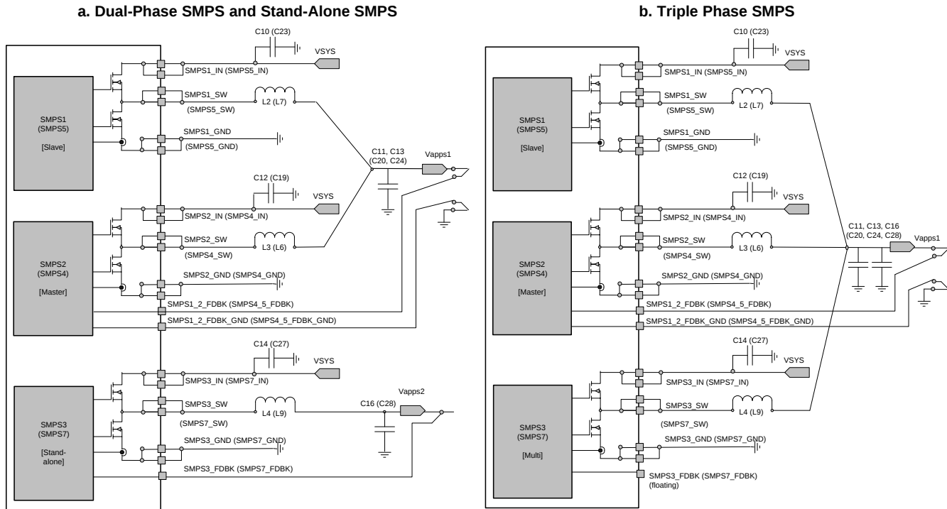
Figure 6-6. Multi-Phase SMPS Connectivity
