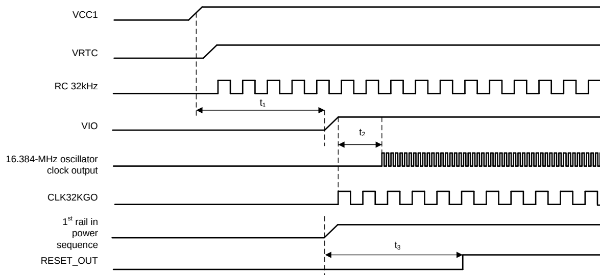
Figure 6-20. Start Up Timing Diagram
