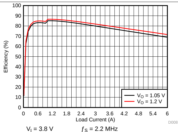
Figure 5-6. SMPS Efficiency for 6-A Multi-Phase PWM Mode
