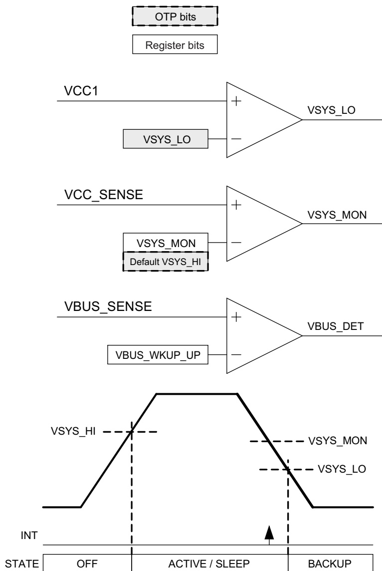
Figure 6-27. System Comparators
