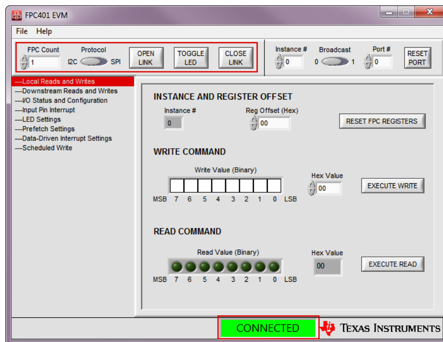
Figure 6. Communication Control
