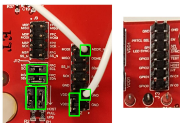
Figure 3. I2C Configuration
