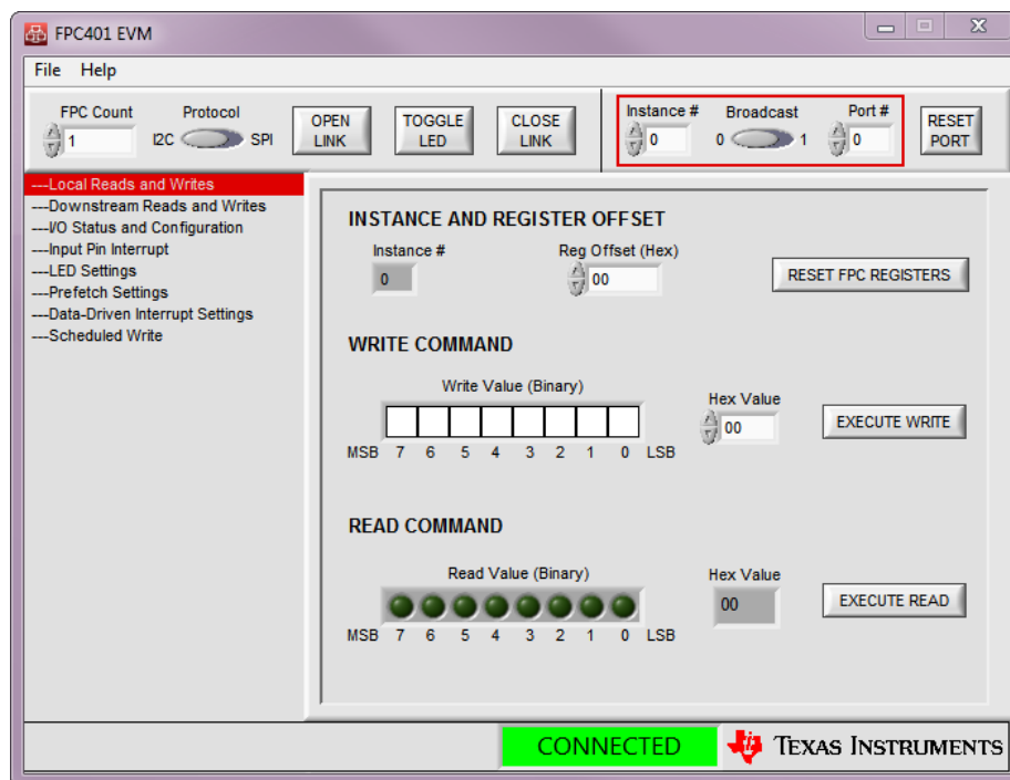
Figure 7. FPC Instance and Port Selection
