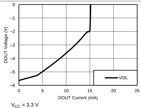
Figure 2. DOUT V_{OL} vs Load Current, Both Drivers Loaded
