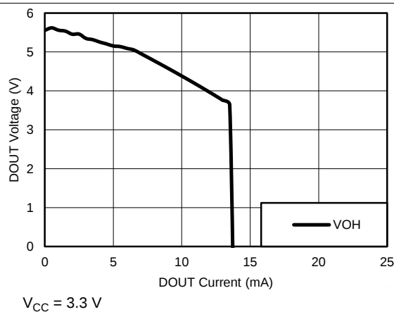
Figure 1. DOUT V_{OH} vs Load Current, Both Drivers Loaded
