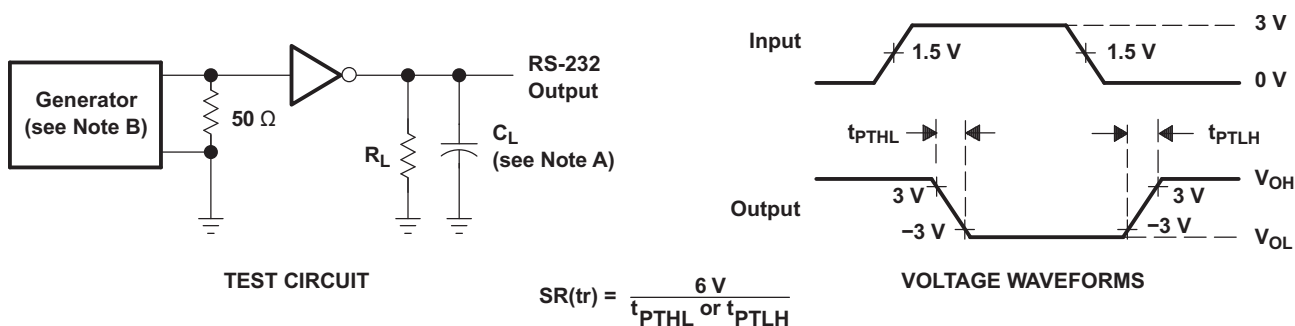
Figure 4. Driver Slew Rate
