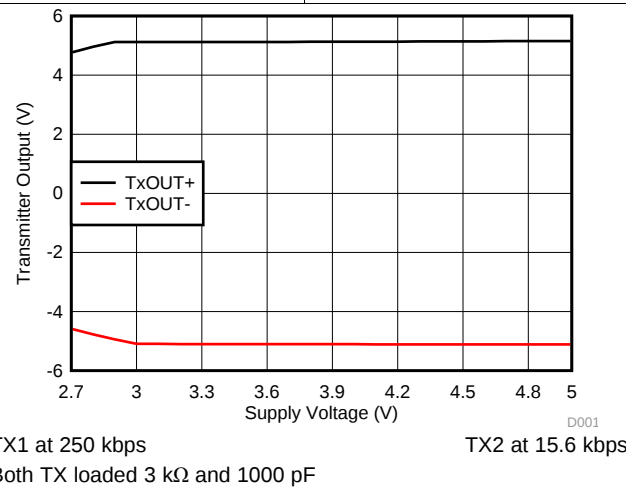
Figure 3. Driver Output Voltage vs. Supply Voltage, Both Drivers Loaded
