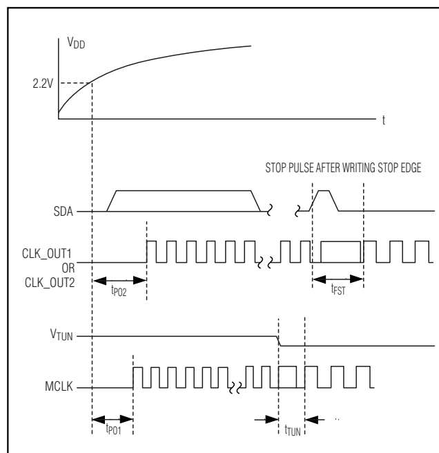
Figure 9. VCXO and PLL Settling Time
