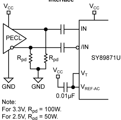
Figure 3d. AC-Coupled PECL Input Interface
