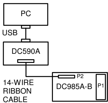
Figure 2. QuickEval Setup
