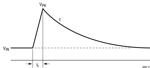
Figure 12. Prototypical Transient Waveform
