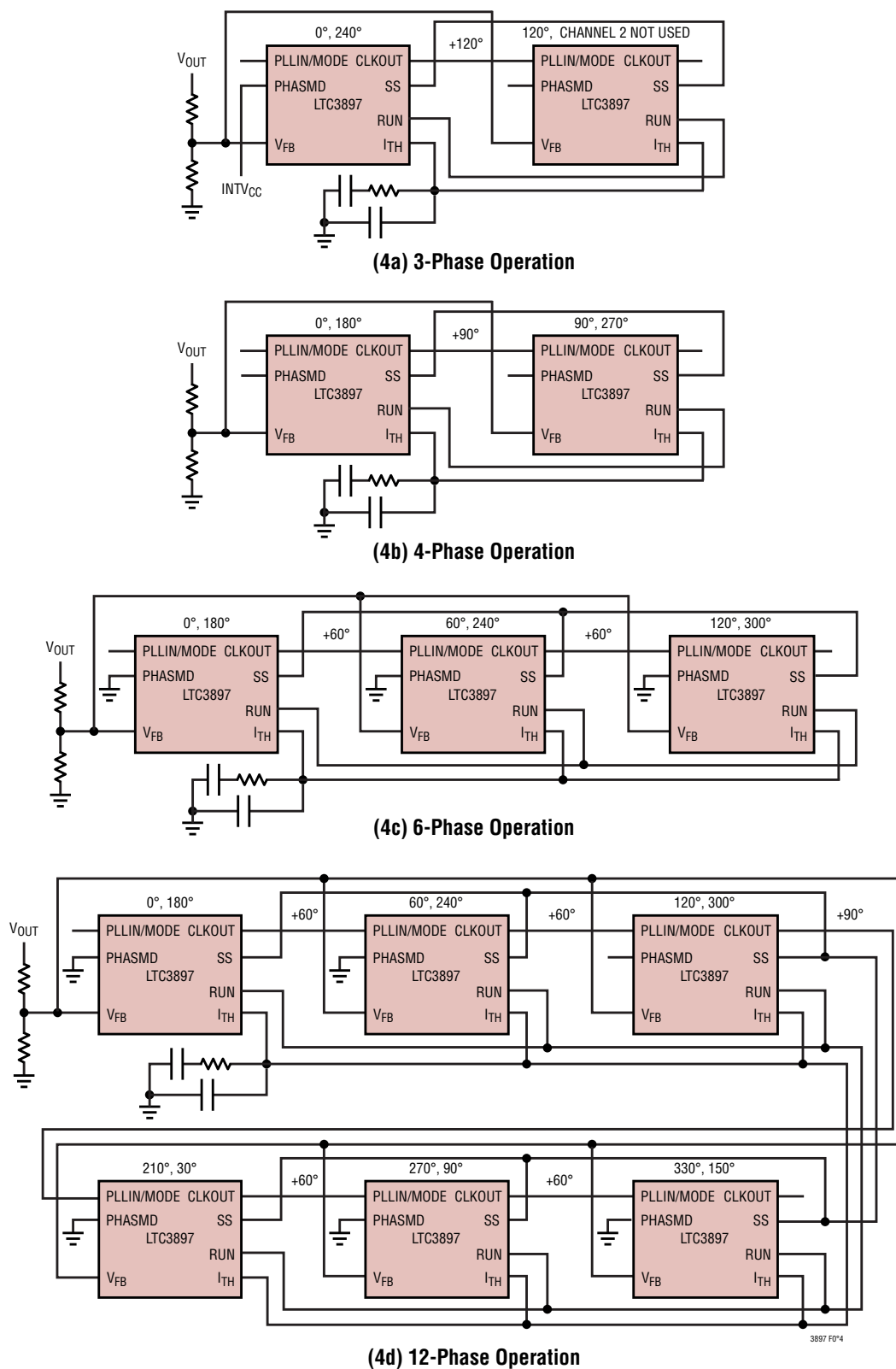
Figure 4. PolyPhase Operation
