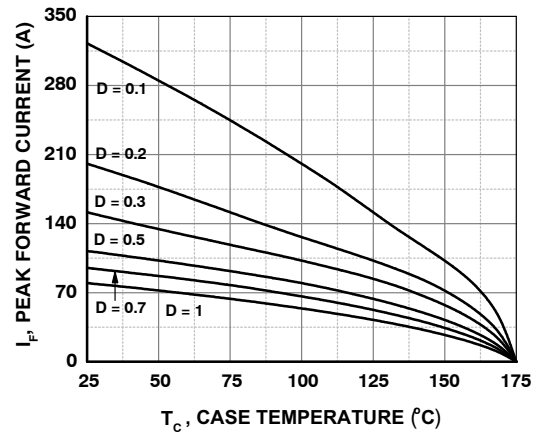
Figure 4. Current Derating
