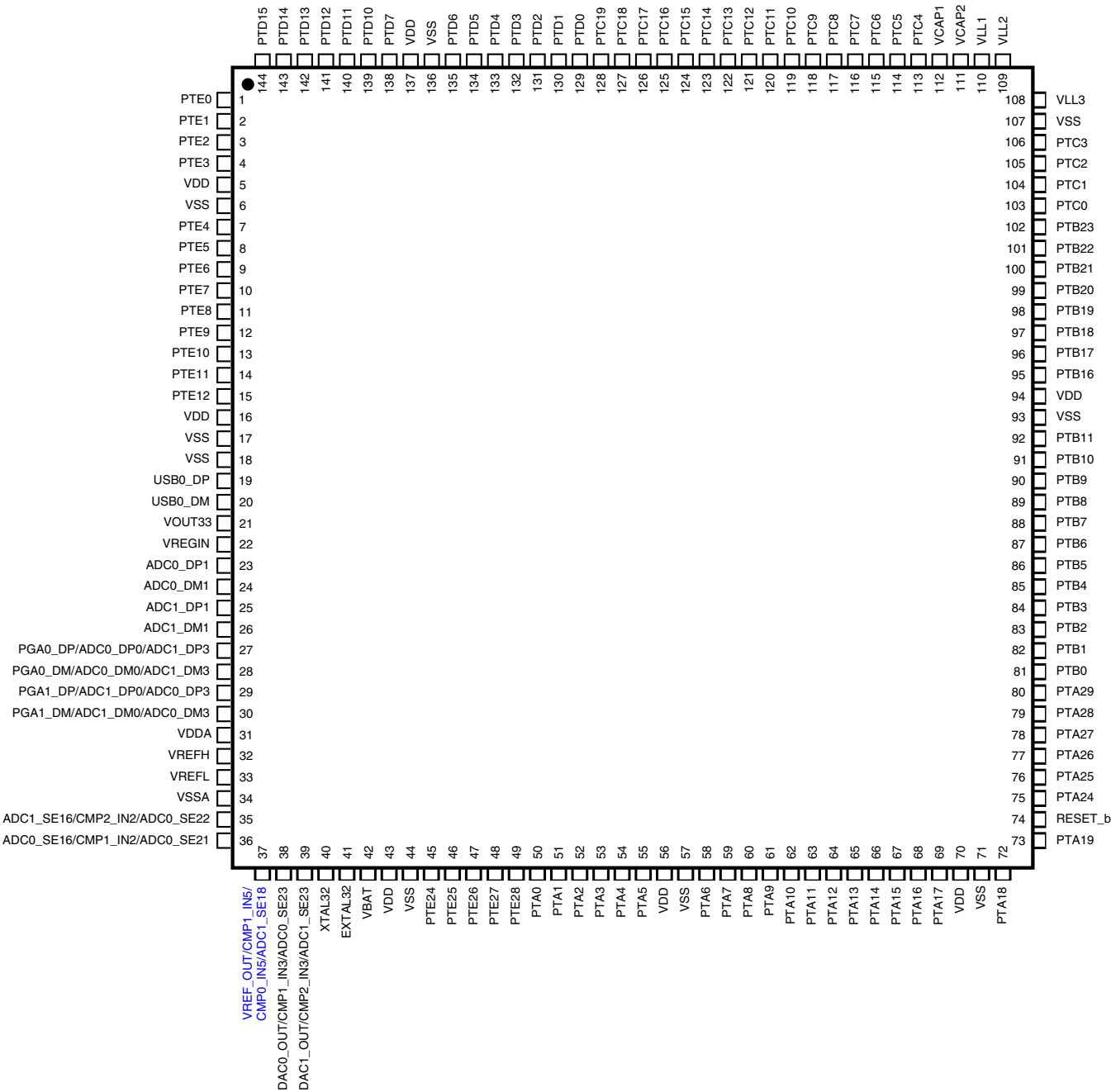
Figure 10-2. K40 144 LQFP Pinout Diagram
