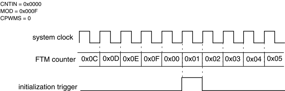
Figure 37-239. Initialization Trigger Is Generated When the FTM Counting Achieves the CNTIN Register Value
