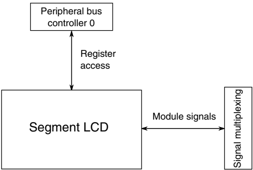
Figure 3-64. SLCD configuration
