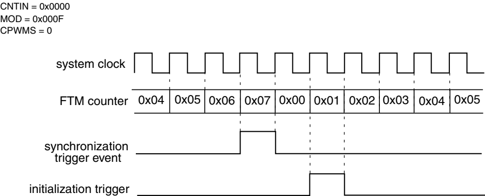
Figure 37-241. Initialization Trigger Is Generated When There Is the FTM Counter Synchronization
