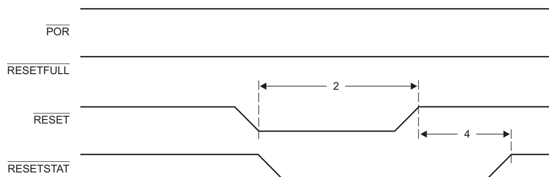
Figure 7-7 Soft/Hard-Reset Timing
