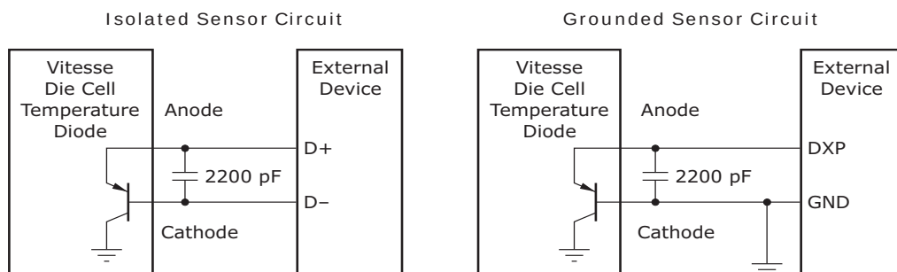
Figure 20 • Thermal Diode
