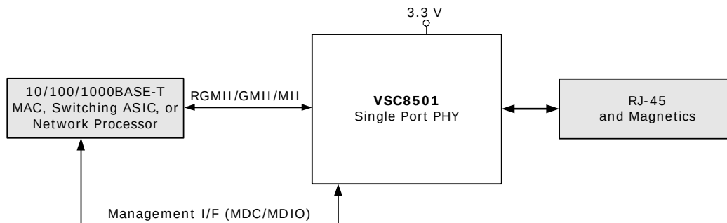
Figure 1 • Copper Transceiver Application Diagram
