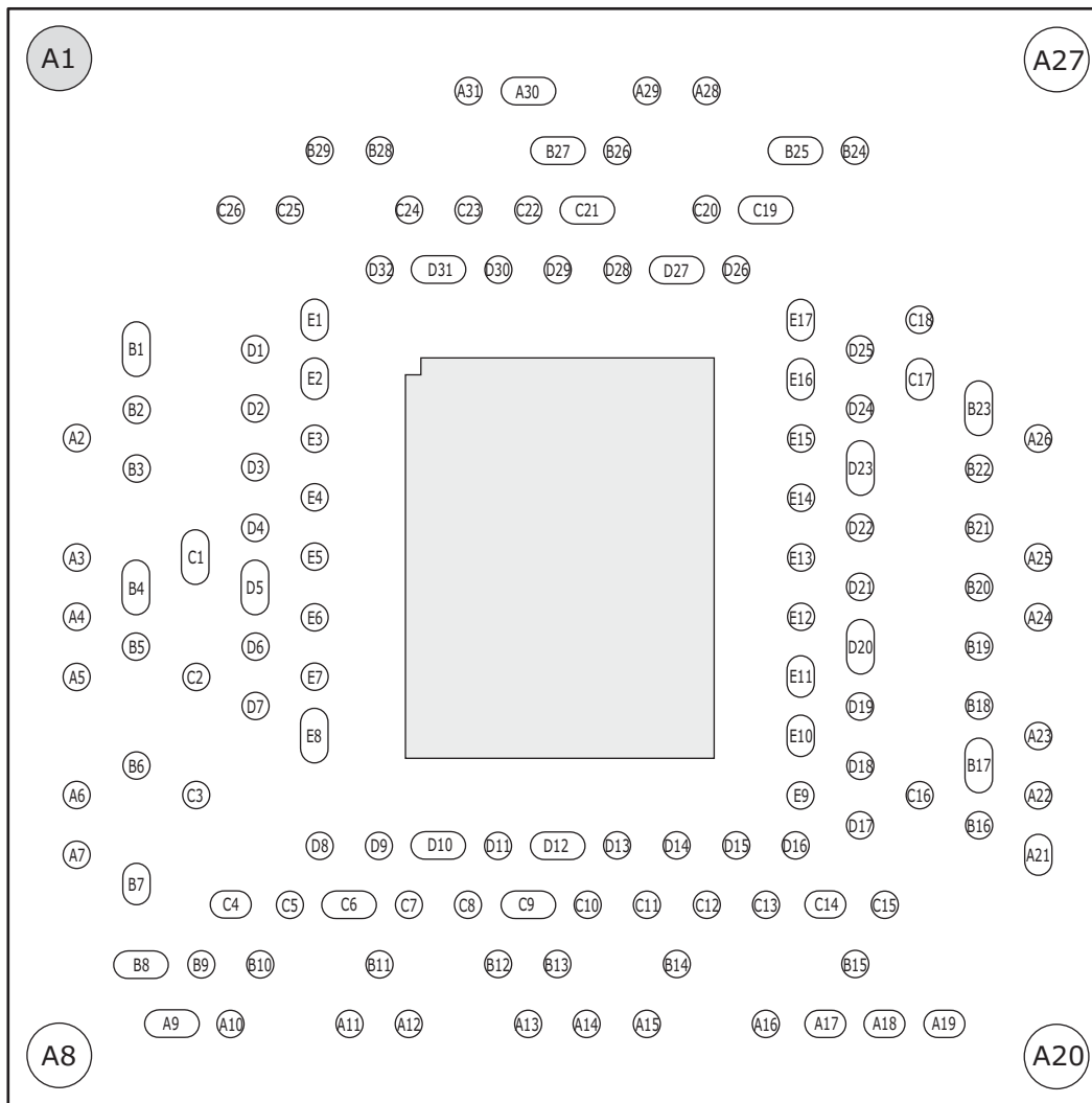
Figure 30 • Pin Diagram
