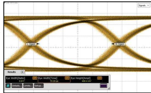
Figure 26. TL = 3-Meter 30-AWG 100 \Omega Twin-Axial Cable, DS100BR111 CHA, 10.3125 Gbps
