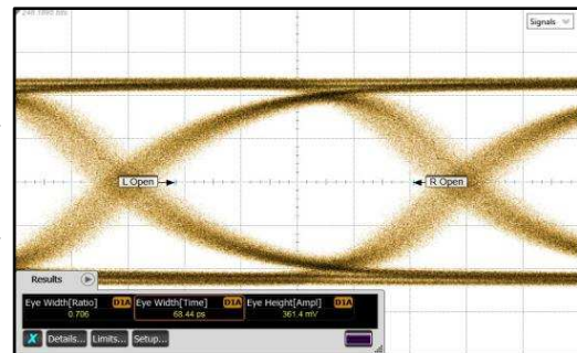
Figure 28. TL = 7-Meter 30-AWG 100 \Omega Twin-Axial Cable, DS100BR111 CHA, 10.3125 Gbps
