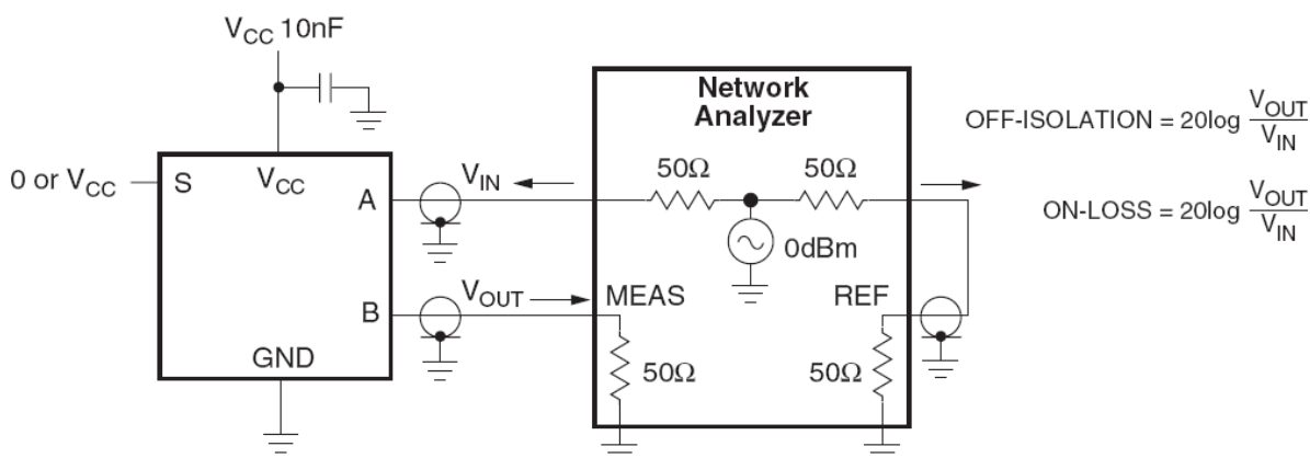
Figure 9. Off Isolation
