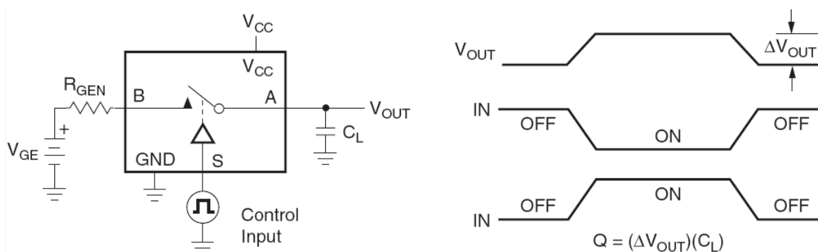
Figure 8. Charge Injection
