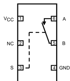
Figure 4. FSA1157 MicroPak™ Top Through View (Normally Closed)
