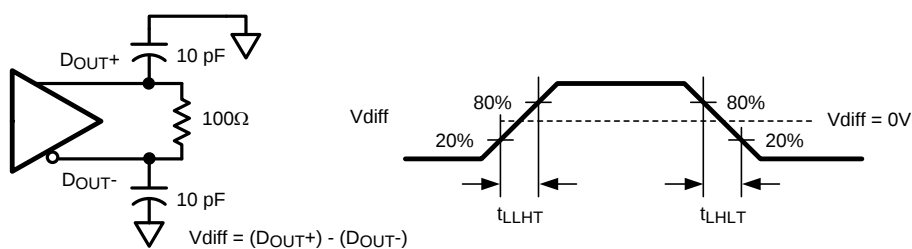
Figure 5. Serializer LVDS Output Load and Transition Times
