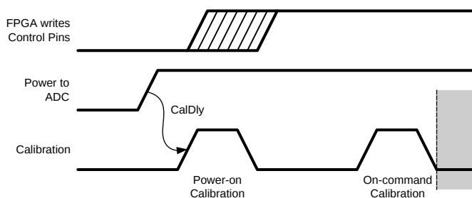
Figure 77. Power-On With Control Pins Set by FPGA Post Power-on Cal
