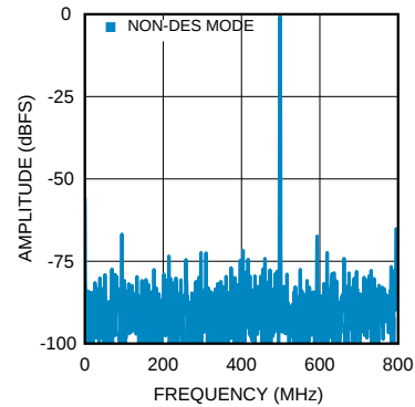
Figure 52. Spectral Response at f_{IN} = 498\text{ MHz} (ADC12D1600)
