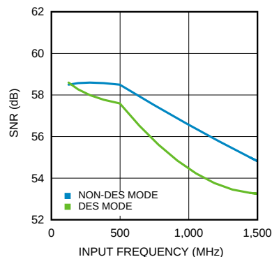
Figure 34. SNR vs Input Frequency (ADC12D1600)
