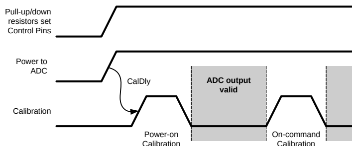
Figure 75. Power-On With Control Pins Set by Pullup and Pulldown Resistors
