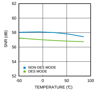
Figure 28. SNR vs Temperature (ADC12D1600)
