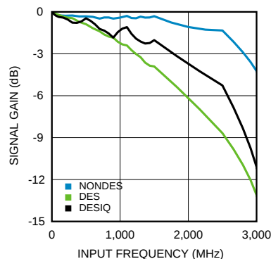
Figure 58. Full Power Bandwidth (ADC12D1600)
