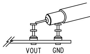
Figure 5. Measuring Output Ripple
