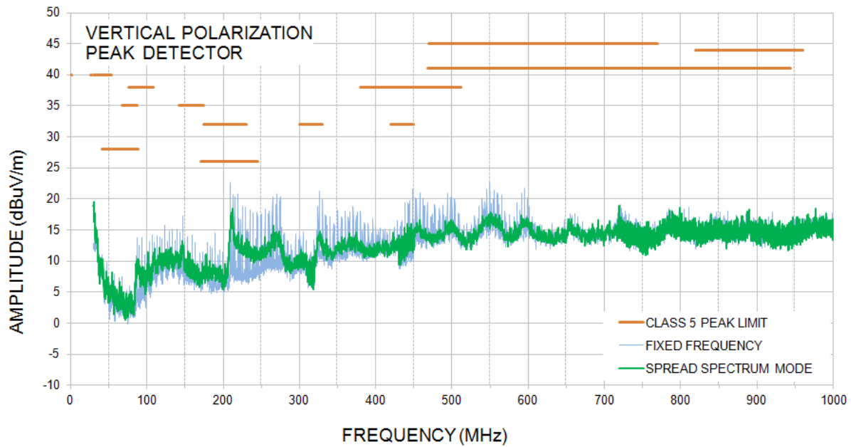
Figure 2. LT8608 Demo Circuit EMI Performance in CISPR25 Radiated Emission Test, Antenna Polarization: Vertical ( V_{IN} = 14V , V_{OUT} = 5V , I_{OUT} = 1.5A , 2MHz Switching Frequency)
