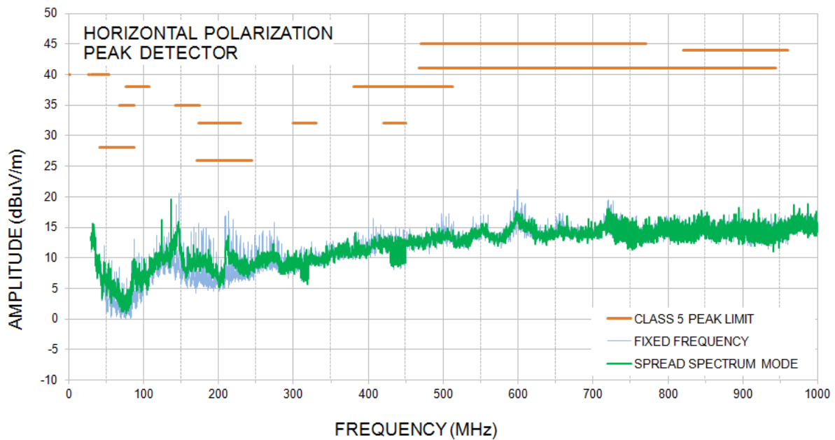
Figure 3. LT8608 Demo Circuit EMI Performance in CISPR25 Radiated Emission Test, Antenna Polarization: Horizontal ( V_{IN} = 14V , V_{OUT} = 5V , I_{OUT} = 1.5A , 2MHz Switching Frequency)
