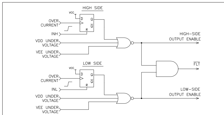
Fig. 4: Logic representation of IXBD4410 \overline{\text{FLT}} signal
