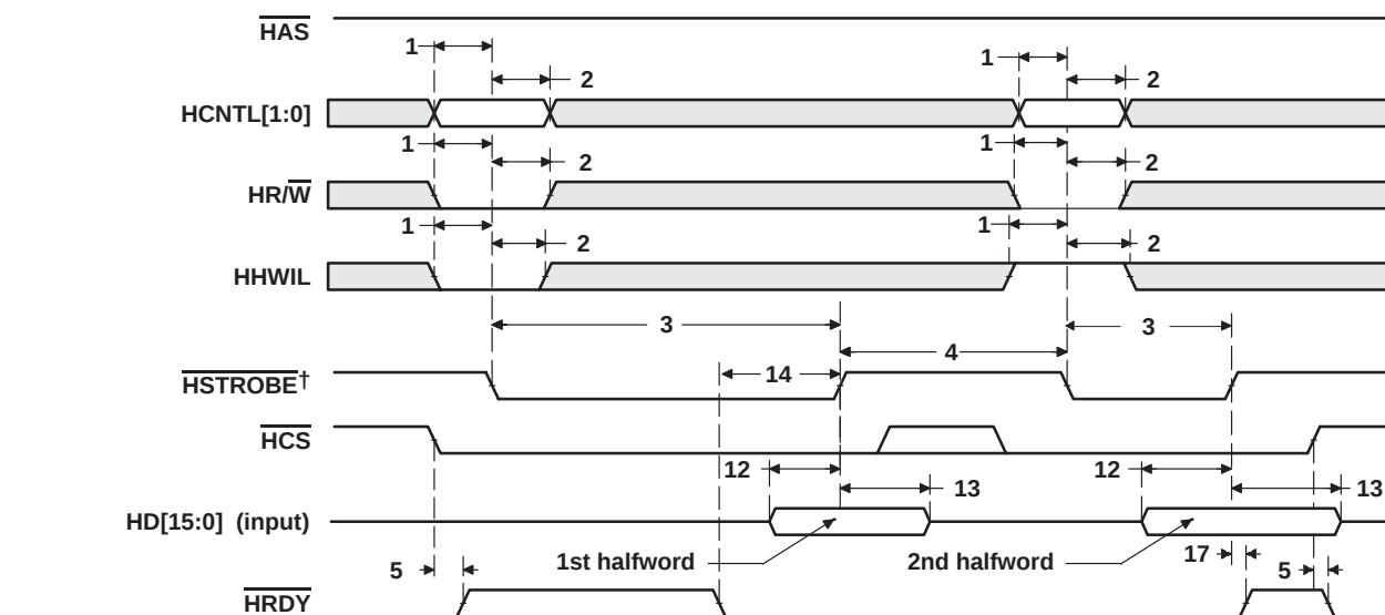
Figure 35. HPI Write Timing ( \overline{HAS} Not Used, Tied High)
