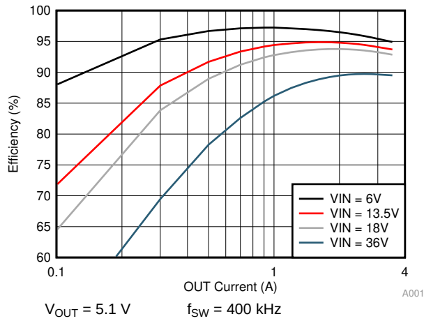
Figure 74. Buck Only Efficiency
