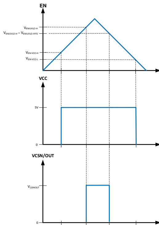
Figure 39. Precision Enable Behavior
