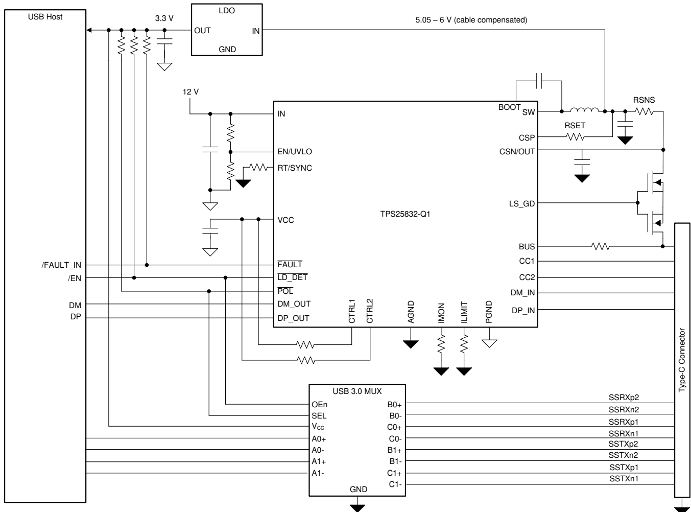
Figure 64. Example Implementation
