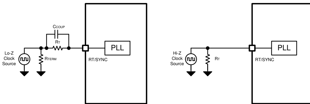
Figure 44. Synchronize to External Clock
