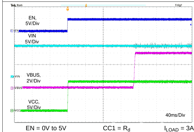
Figure 90. Startup Relate to EN
