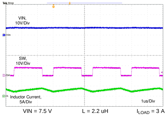
Figure 45. Switching Frequency when R_T = 8.87\text{ k}\Omega
