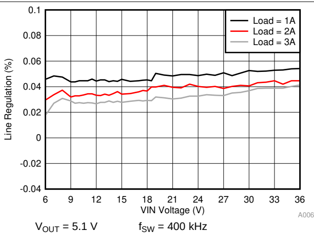
Figure 79. Line Regulation
