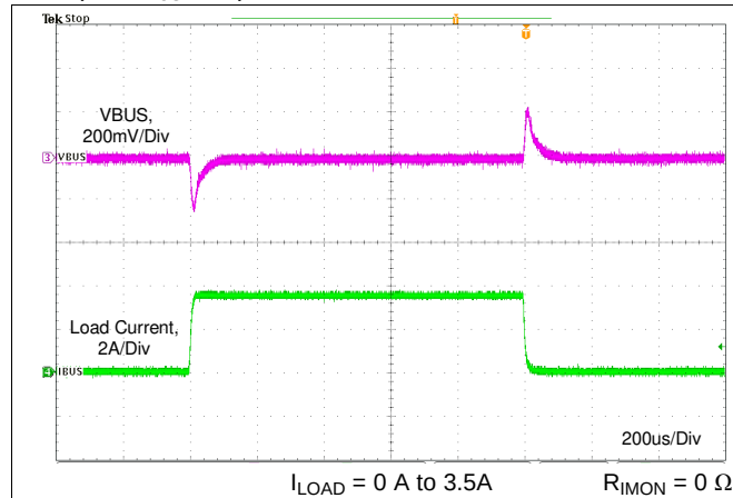
Figure 80. Load Transient Without Cable Compensation
