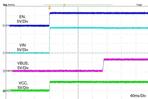
Figure 41. Typical Start-up Behavior, V_{IN} = 13.5 \text{ V} , CC1 = R_d , R_{IMON} = 12.6 \text{ k}\Omega
