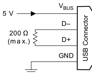
Figure 69. DCP Supporting BC1.2 and YD/T 1591-2009
