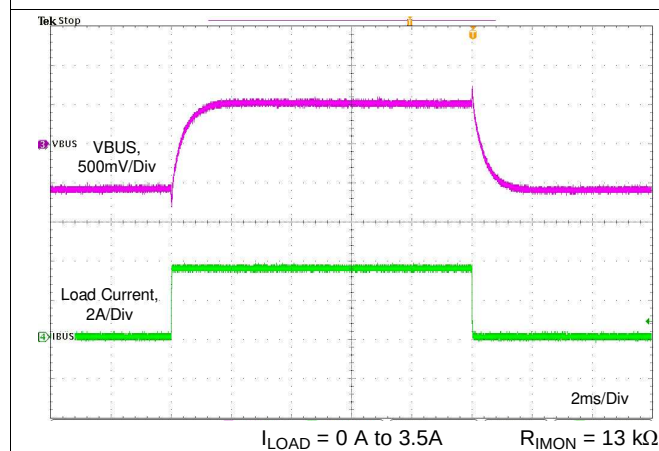
Figure 82. Load Transient With Cable Compensation
