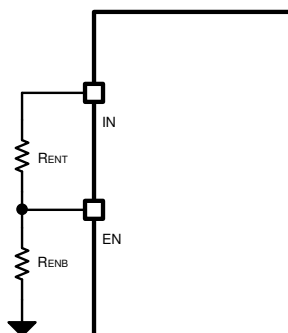
Figure 40. System UVLO by Enable Divider
