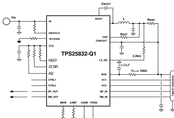
Figure 58. Buck Average Current Limit
