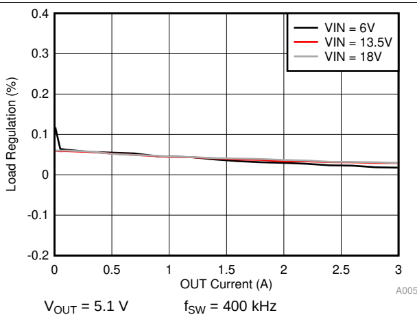
Figure 78. Load Regulation
