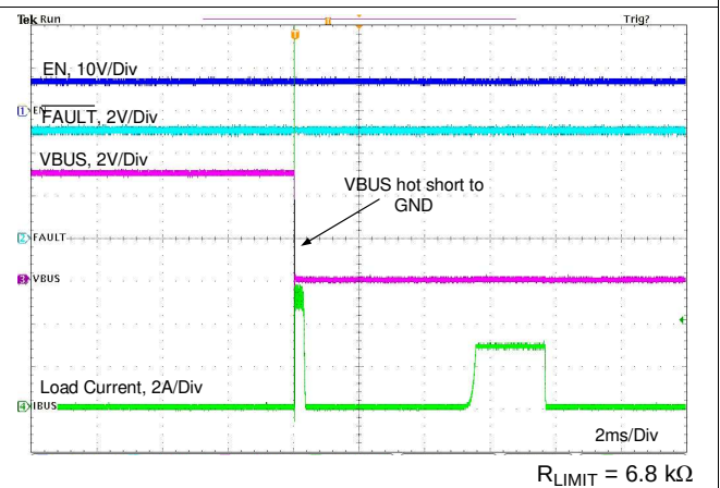
Figure 101. VBUS Hot Short to GND With External FET
