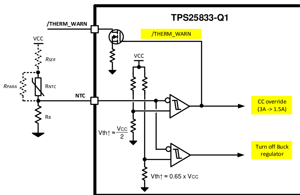
Figure 65. NTC Input Pin
