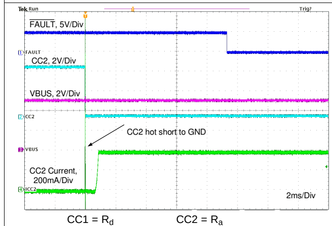
Figure 102. CC2 Hot Short to GND
