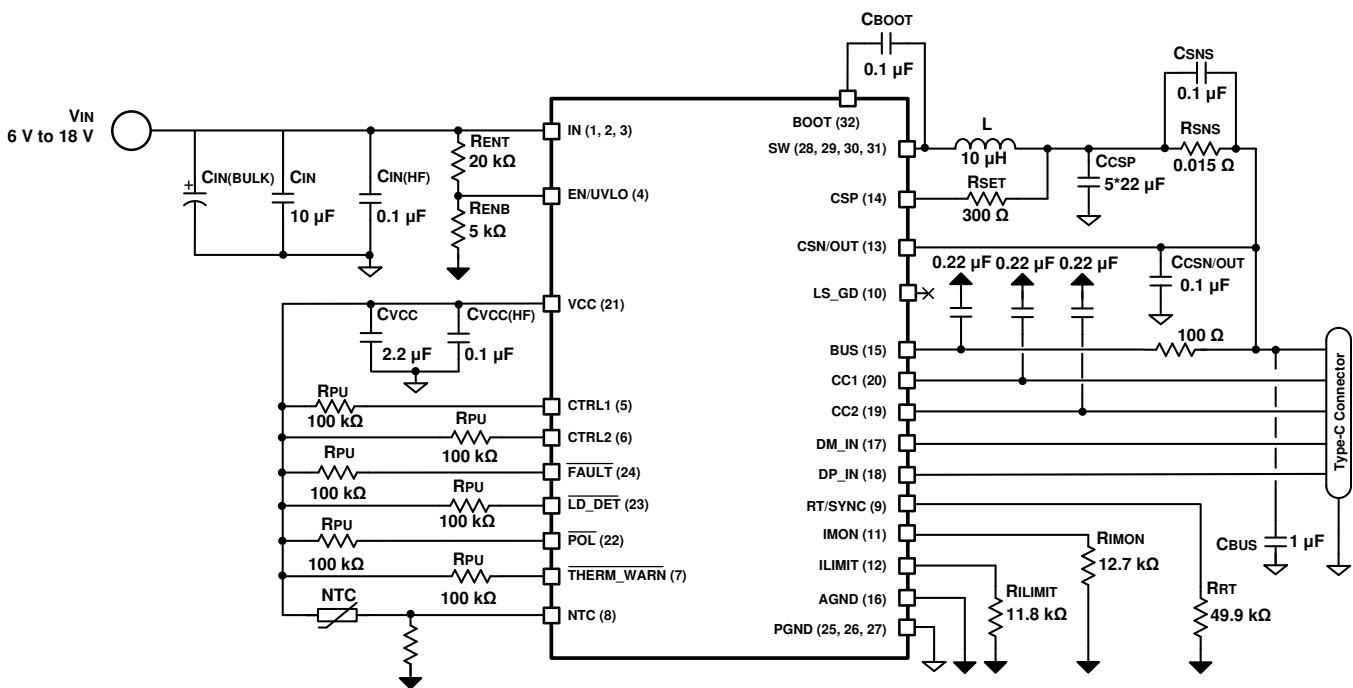
Figure 73. Application Circuit
