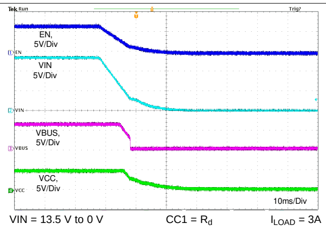
Figure 89. Shutdown Relate to VIN
