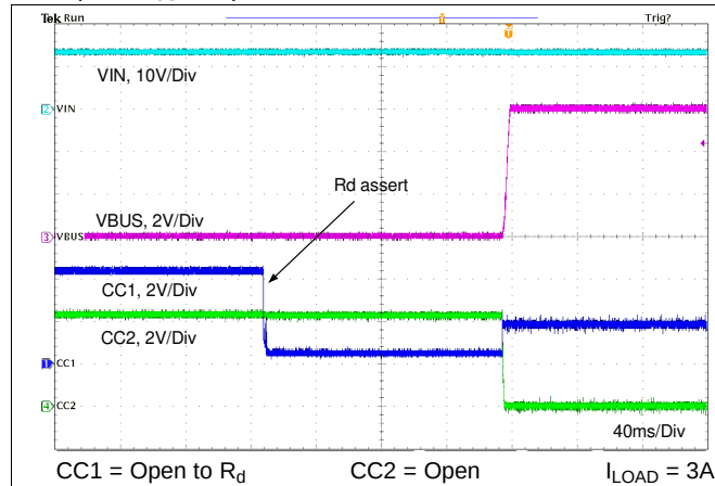
Figure 92. Rd Assert
