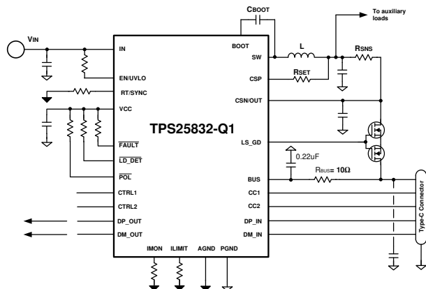
Figure 57. Current Limit with External MOSFET
