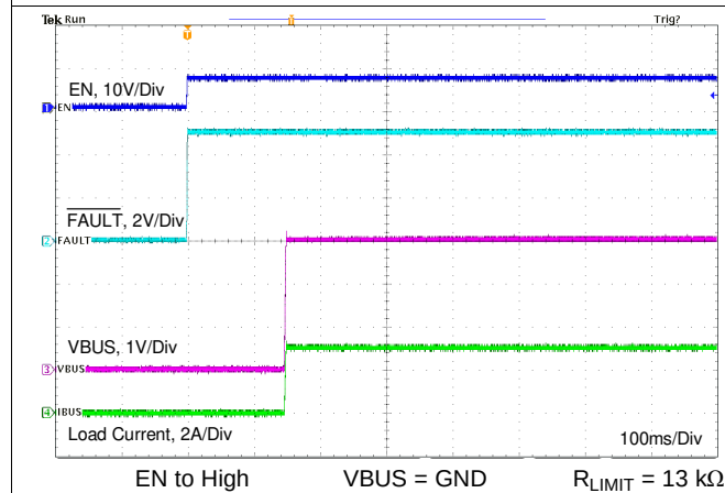
Figure 96. Enable into 1-Ω Load Without External FET
