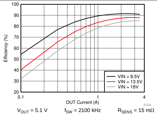
Figure 77. Efficiency with Sense Resistor
