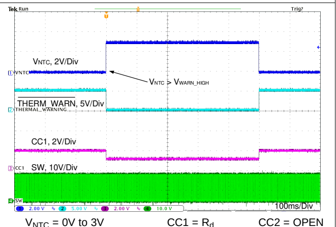
Figure 103. Thermal Sensing with NTC Behavior 1
