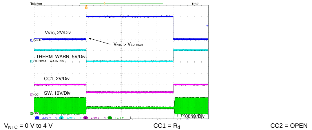
Figure 104. Thermal Sensing with NTC Behavior 2
