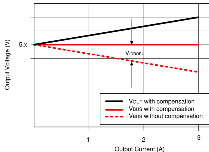
Figure 60. Voltage Drop
