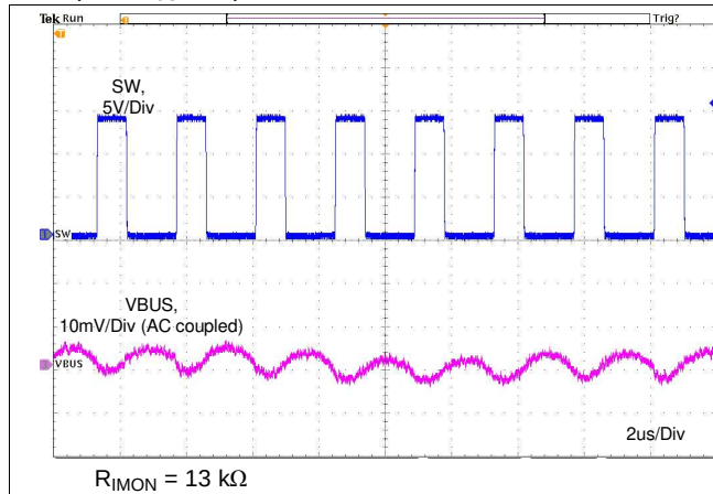
Figure 86. 100-mA Output Ripple
