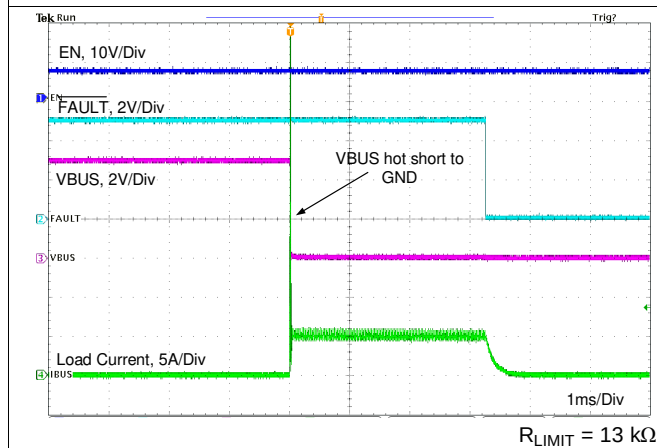
Figure 100. VBUS Hot Short to GND Without External FET
