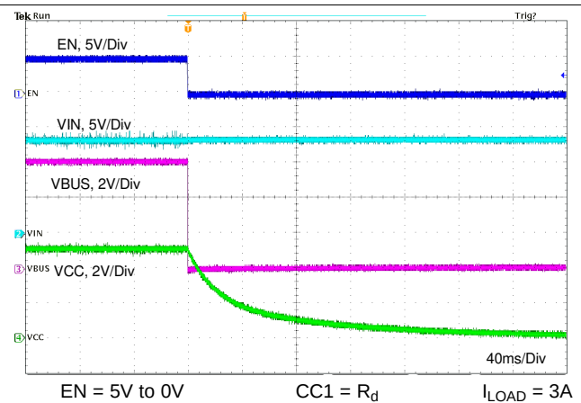
Figure 91. Shutdown Relate to EN
