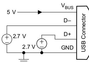
Figure 70. Divider 3 Mode
