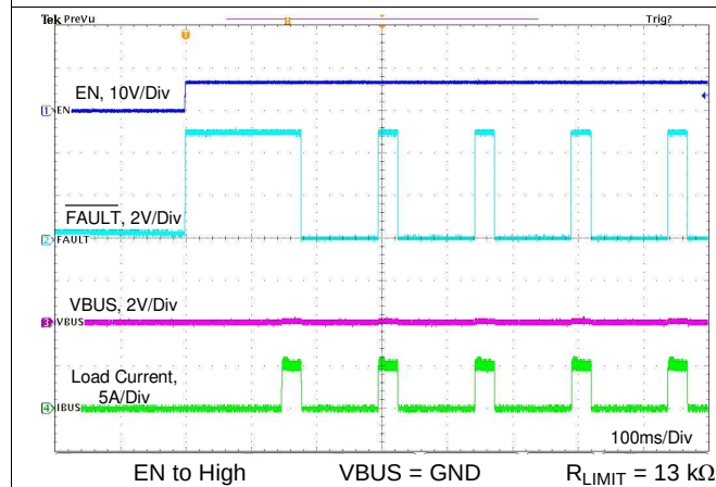
Figure 94. Enable into Short Without External FET
