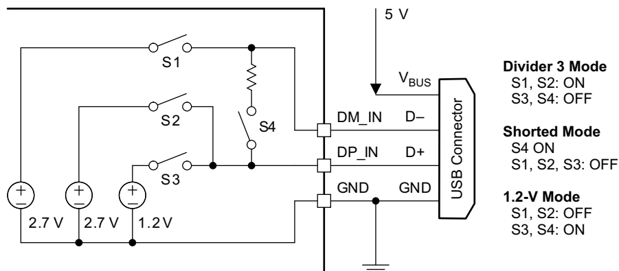
Figure 72. DCP Auto Mode
