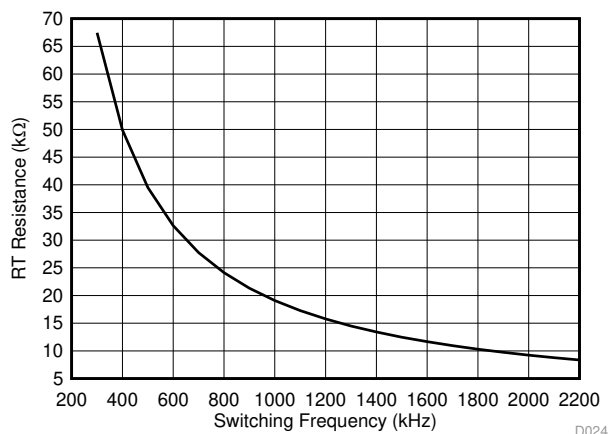
Figure 43. RT Set Resistor vs Switching Frequency
