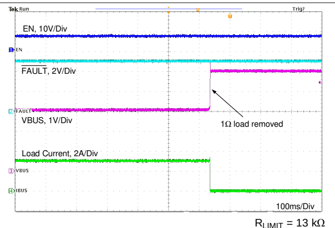
Figure 97. 1-Ω Load Recovery Without External FET
