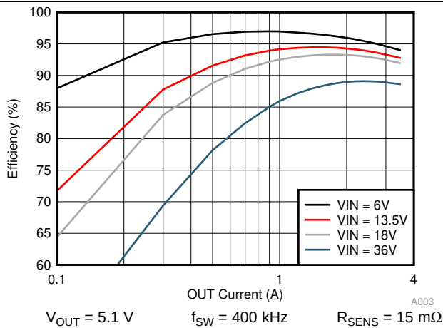
Figure 76. Efficiency with Sense Resistor
