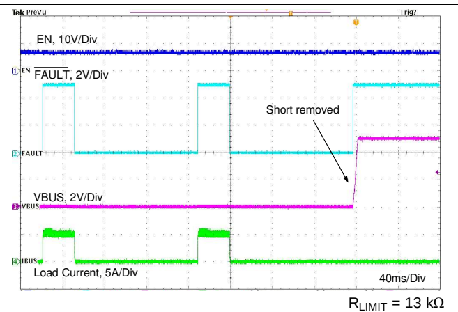
Figure 95. Short Circuit Recovery Without External FET
