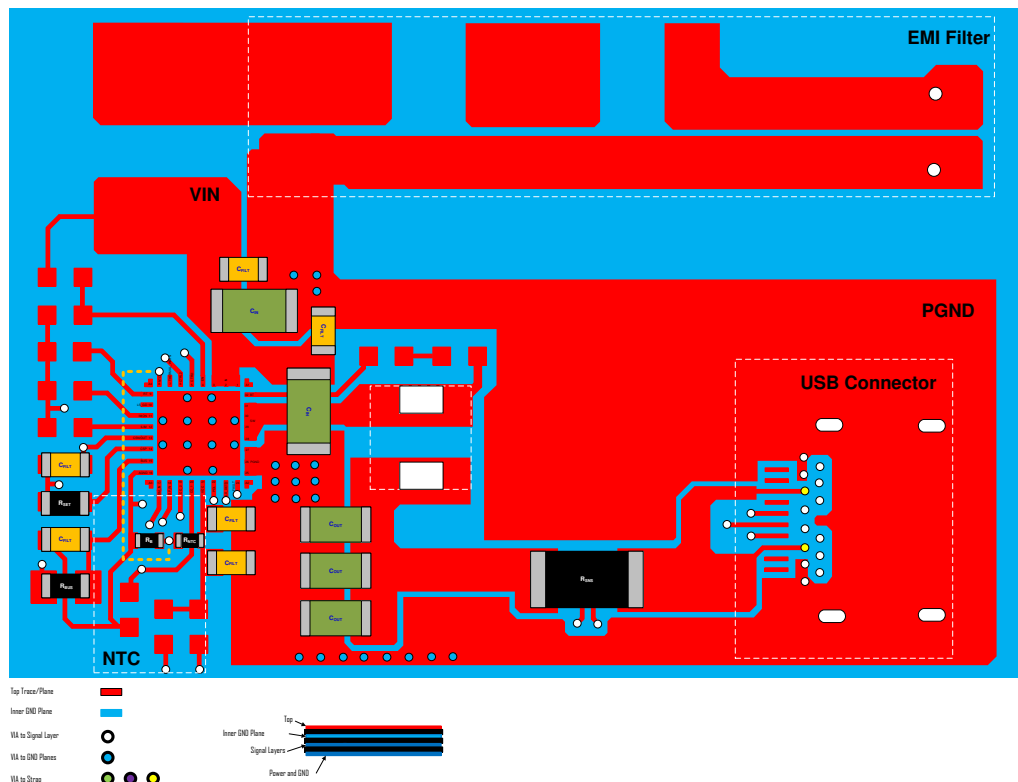
Figure 68. NTC Placement Example
