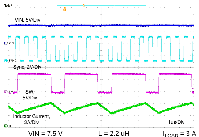
Figure 48. Synchronizing to External 2.1MHz Clock
