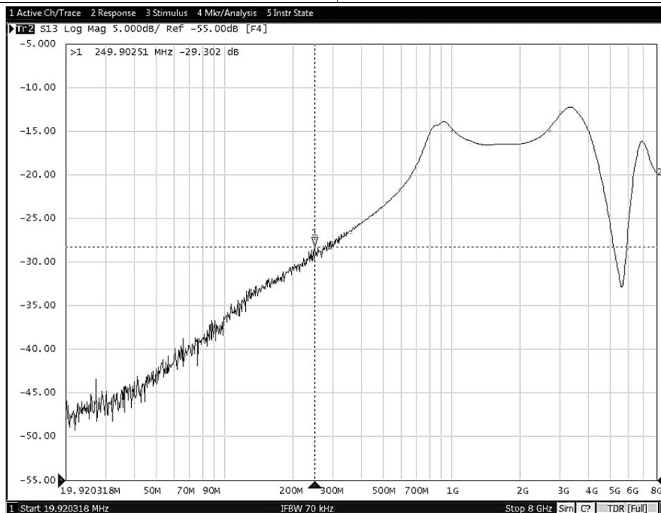
Figure 31. Data Transmission Characteristics vs Frequency (TPS25832-Q1)
