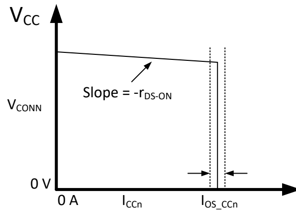
Figure 63. VCONN Current Limit Profile
