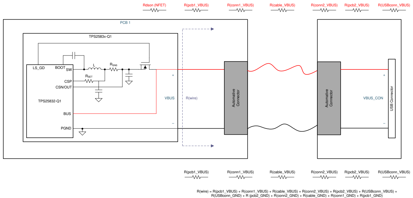
Figure 59. Automotive USB Resistances
