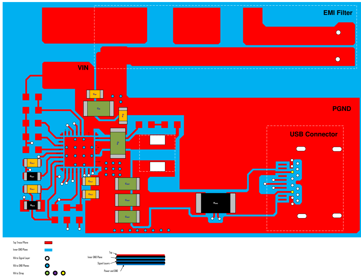
Figure 105. Layout
