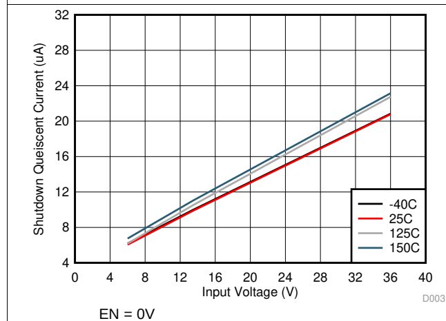
Figure 3. Shutdown Quiescent Current
