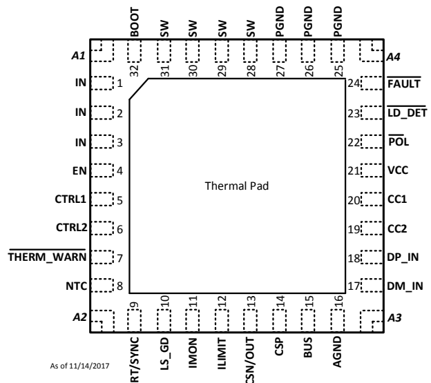
TPS25833-Q1 RHB Package 32-Pin (VQFN) Top View
