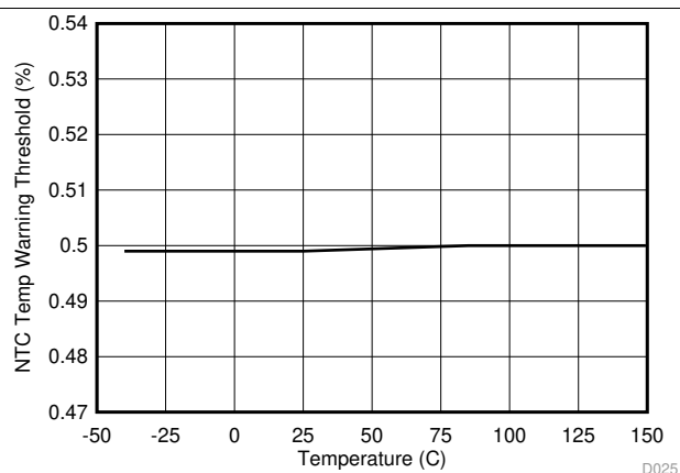
Figure 27. NTC Temperature Warning Threshold (TPS25833-Q1)
