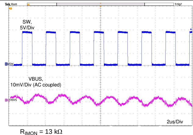
Figure 85. 3.5-A Output Ripple
