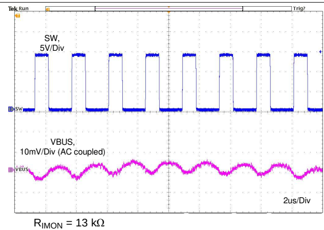
Figure 87. No Load Output Ripple
