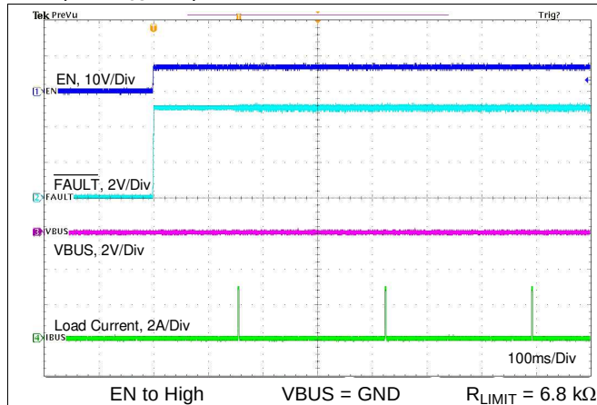
Figure 98. Enable into Short With External FET
