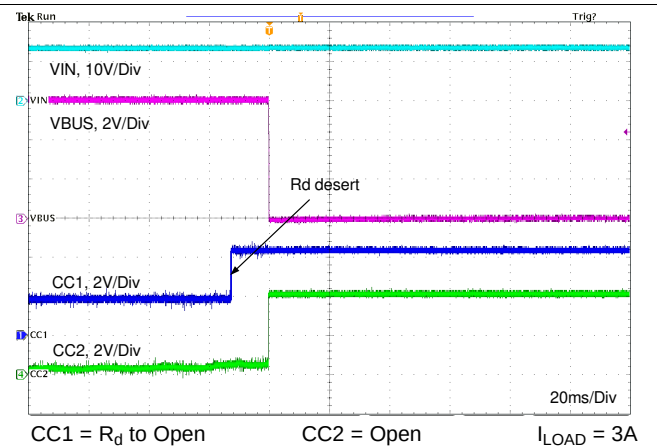
Figure 93. Rd Desert
