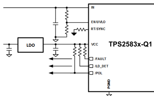
Figure 51. V CONN Source Using External LDO
