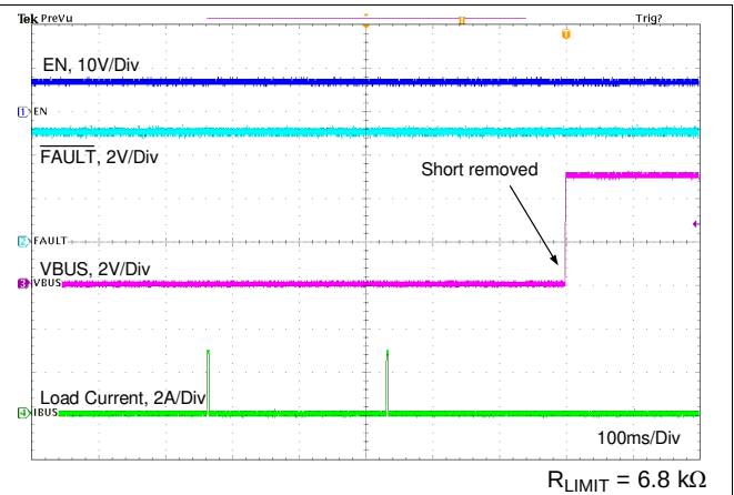
Figure 99. Short Circuit Recovery With External FET
