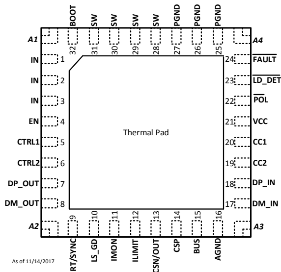
TPS25832-Q1 RHB Package 32-Pin (VQFN) Top View
