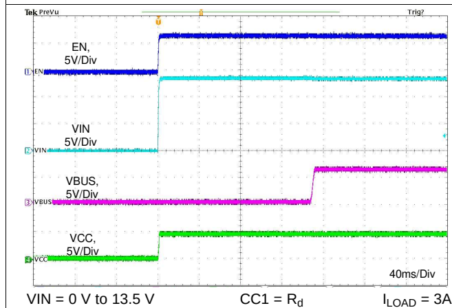
Figure 88. Startup Relate to VIN
