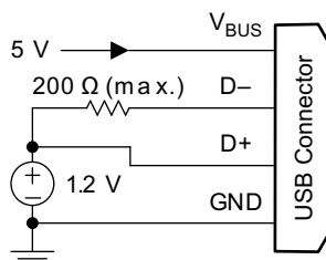
Figure 71. 1.2-V Mode
