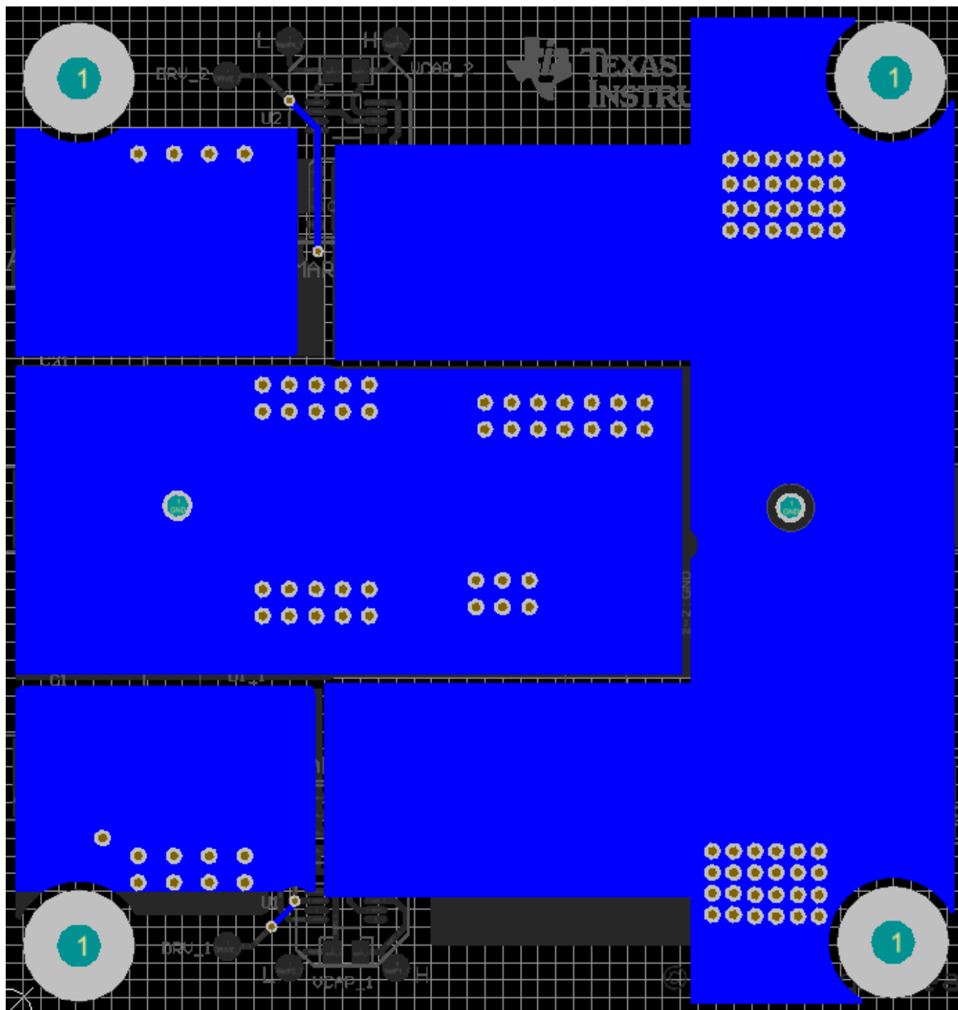
Figure 8. Bottom Layer
