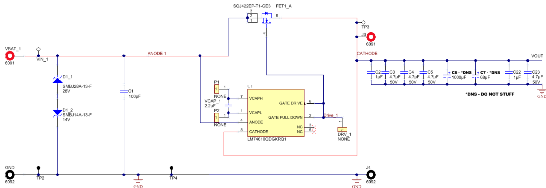
Figure 9. LM74610-SQEVm Schematic
