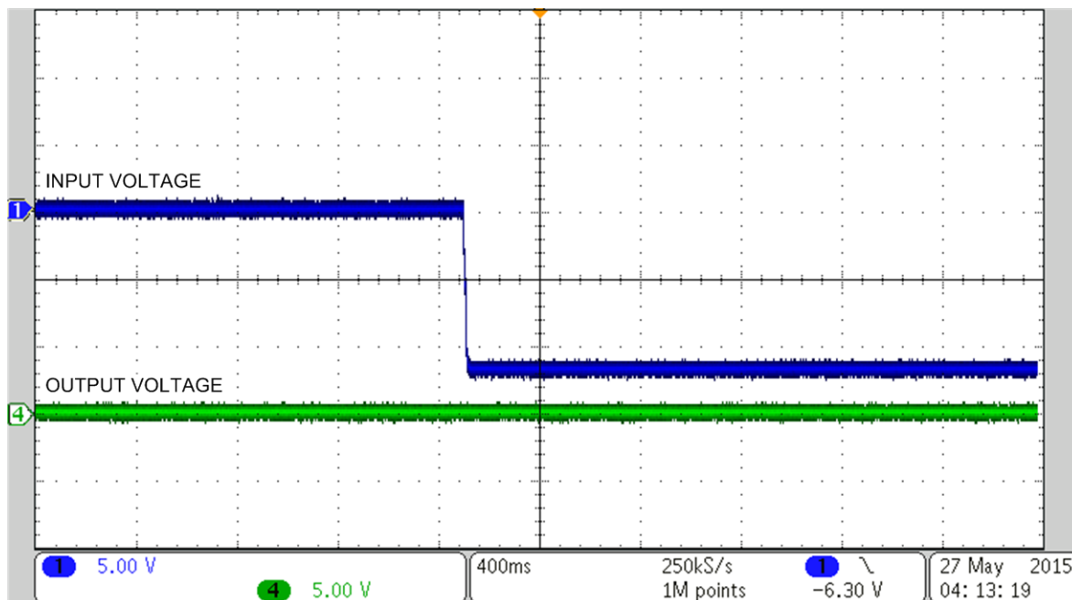
Figure 4. Response to Start Up Reverse Polarity
