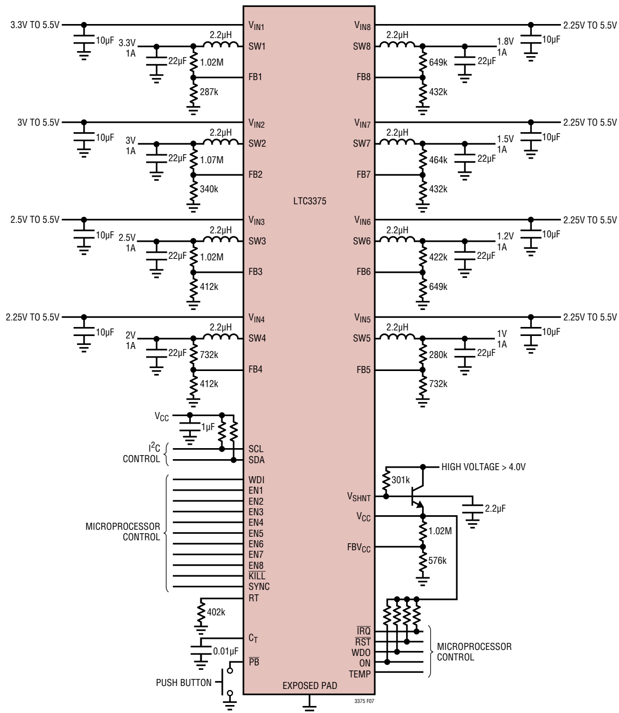
Figure 7. Detailed Front Page Application Circuit
