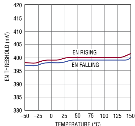
Enable Pin Precision Threshold vs Temperature
