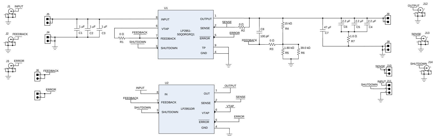
Figure 10. LP2951EVM Schematic
