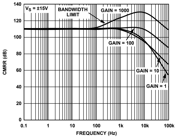
Figure 28. CMRR vs. Frequency, RTI, V_S = \pm 15V
