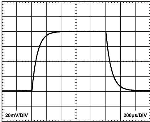
Figure 53. Small Signal Pulse Response, G = 100 , R_L = 20\text{ k}\Omega , C_L = 100\text{ pF}
