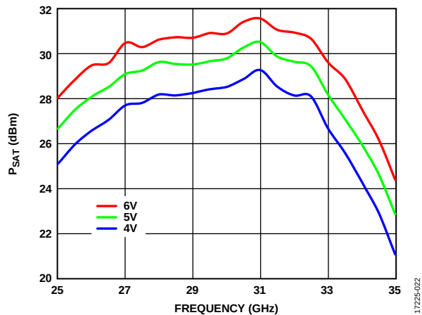
Figure 22. P_{SAT} vs. Frequency for Various Drain Bias Voltages ( V_{DDX} ), I_{DDQ} = 650\text{ mA}
