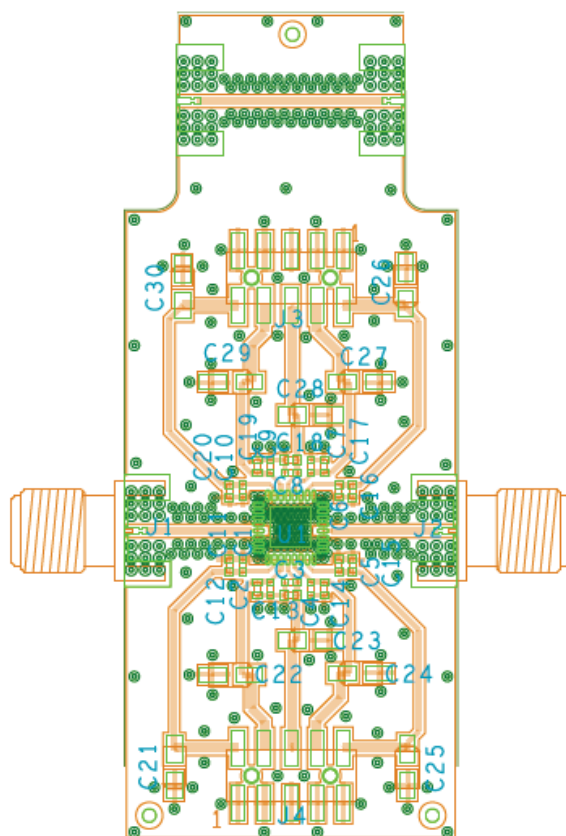
Figure 50. Evaluation PCB
