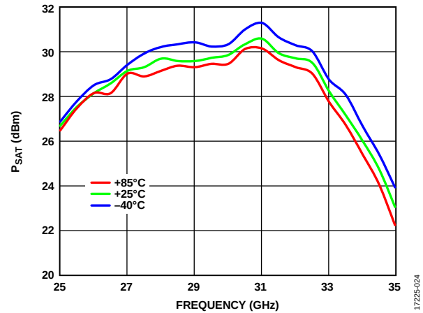
Figure 24. P_{SAT} vs. Frequency for Various Temperatures, V_{DDX} = 5\text{ V} , I_{DDQ} = 650\text{ mA}
