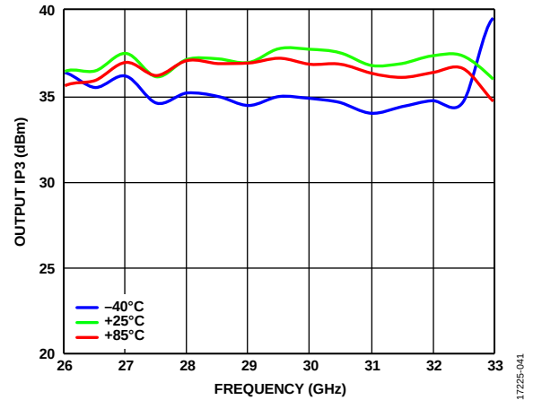
Figure 41. Output IP3 vs. Frequency for Various Temperatures, P_{OUT}\text{ per Tone} = 20\text{ dBm} , V_{DDx} = 5\text{ V} , I_{DDQ} = 650\text{ mA}
