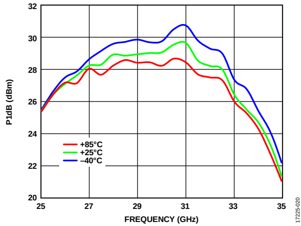
Figure 20. P1dB vs. Frequency for Various Temperatures, V_{DDX} = 5\text{ V} , I_{DDQ} = 650\text{ mA}
