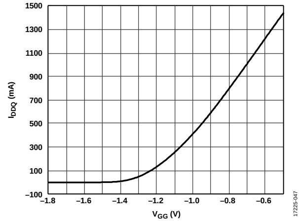
Figure 47. Quiescent Current ( I_{DDQ} ) vs. V_{GG} , V_{DDX} = 5\text{ V} , Representative of a Typical Device
