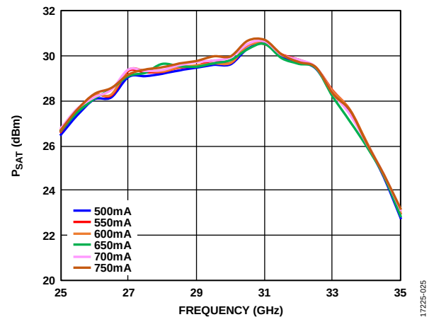
Figure 25. P_{SAT} vs. Frequency for Various Quiescent Currents ( I_{DDQ} ), V_{DDX} = 5\text{ V}
