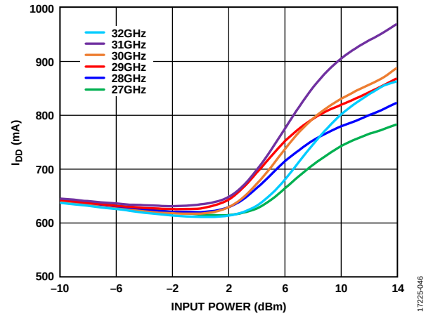
Figure 46. Drain Current ( I_{DD} ) vs. Input Power for Various Frequencies, V_{DDX} = 5\text{ V} , I_{DDQ} = 650\text{ mA}
