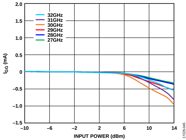
Figure 45. Gate Current ( I_{GG} ) vs. Input Power for Various Frequencies, V_{DDX} = 5\text{ V} , I_{DDQ} = 650\text{ mA}
