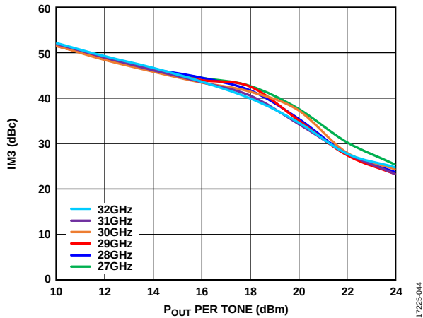
Figure 44. IM3 vs. P_{OUT} per Tone, V_{DDX} = 6\text{ V} , I_{DDQ} = 650\text{ mA}
