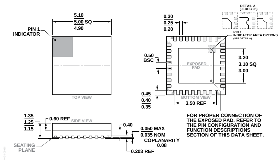
Figure 52. 32-Lead Lead Frame Chip Scale Package, Premolded Cavity [LFCSP_CAV] 5 mm × 5 mm Body and 1.25 mm Package Height (CG-32-2)
