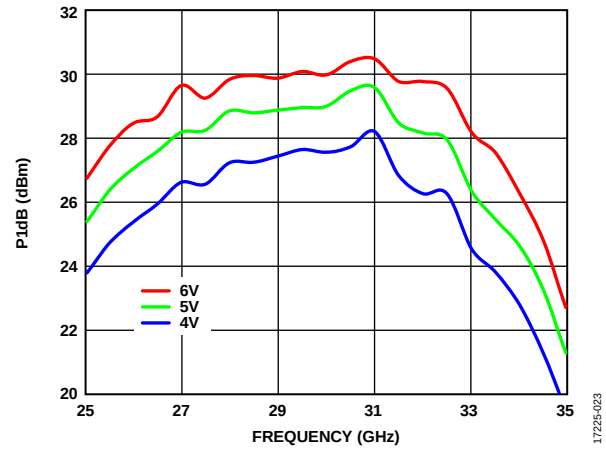
Figure 23. P1dB vs. Frequency for Various Drain Bias Voltages ( V_{DDX} ), I_{DDQ} = 650\text{ mA}
