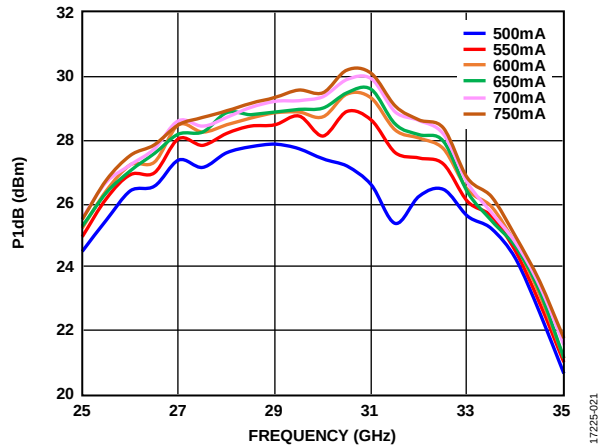
Figure 21. P1dB vs. Frequency for Various Quiescent Currents ( I_{DDQ} ), V_{DDX} = 5\text{ V}
