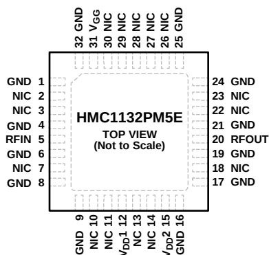
Figure 2. Pin Configuration
