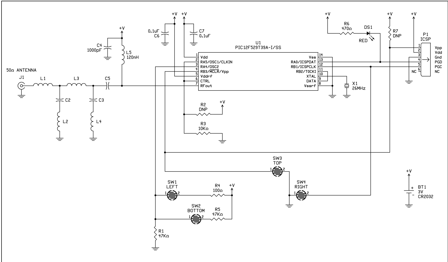
FIGURE 9-8: APPLICATION SCHEMATIC
