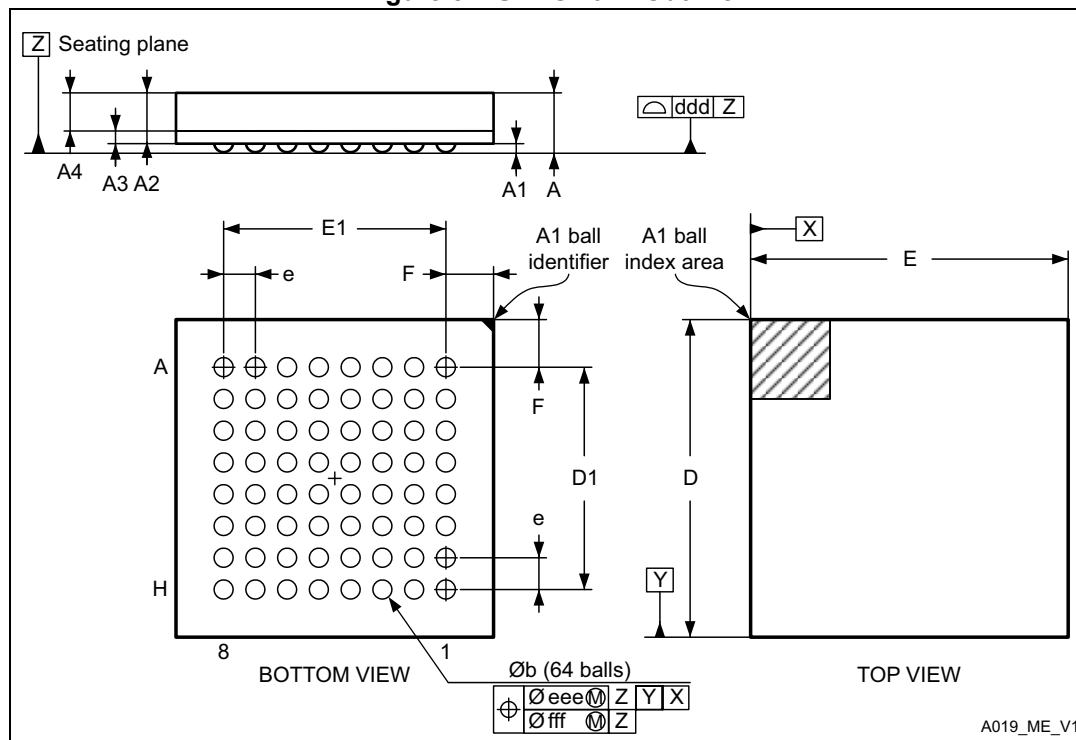
Figure 51. UFBGA64 - Outline
