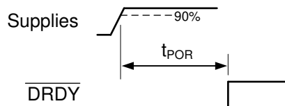
Figure 3. Power-On-Reset Timing
