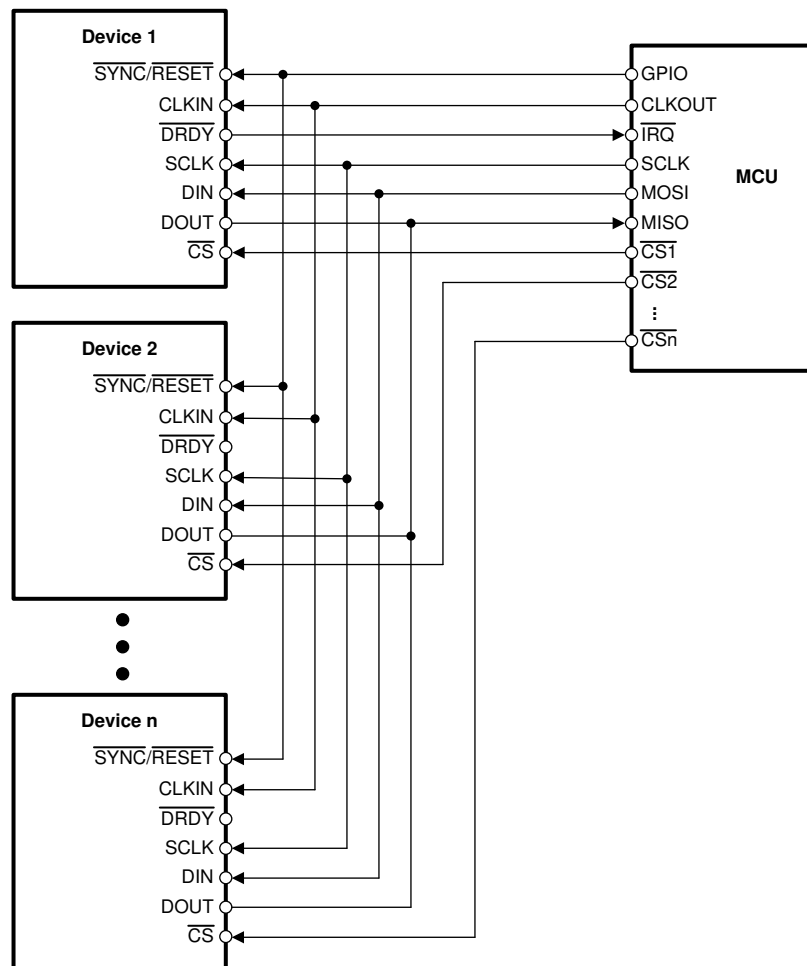
Figure 86. Multiple Device Configuration
