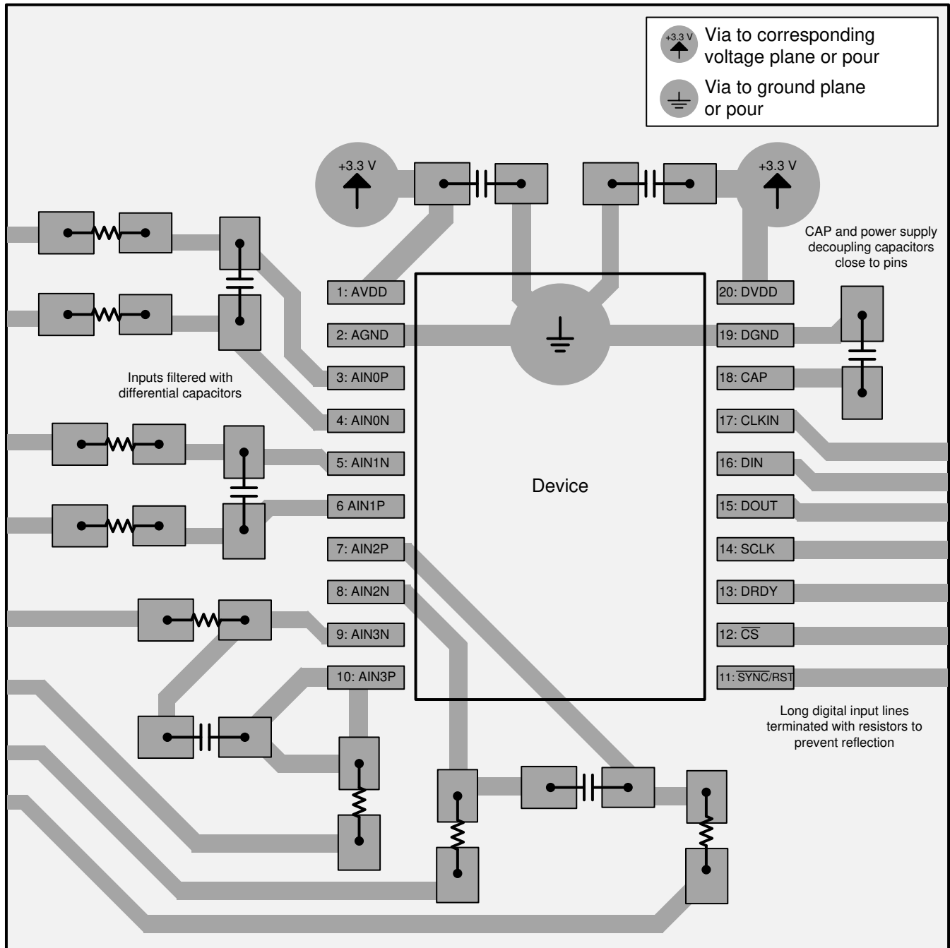
Figure 92. Layout Example
