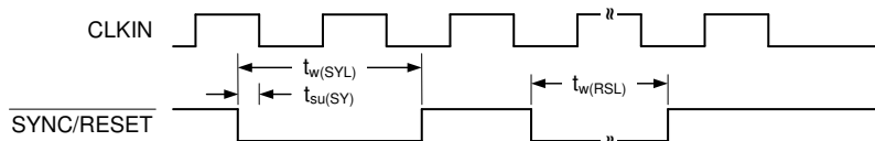
Figure 2. SYNC/RESET Timing Requirements
