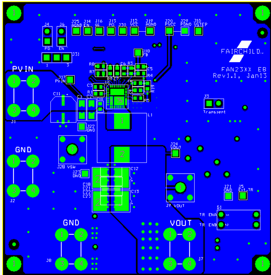
Figure 30. Evaluation Board Top Layer Copper
