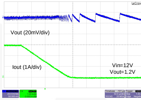
Figure 18. FAN2306M Transition from CCM to DCM
