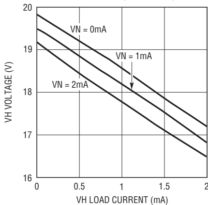
VH Voltage vs VH and VN Load Current (FBN = 0V)
