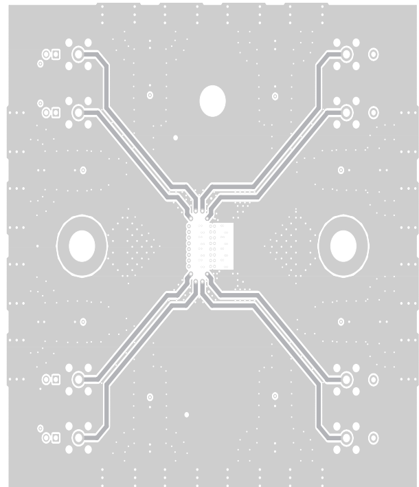
Figure 17. TMS4524EVM: Ground Layer (Layer 2)
