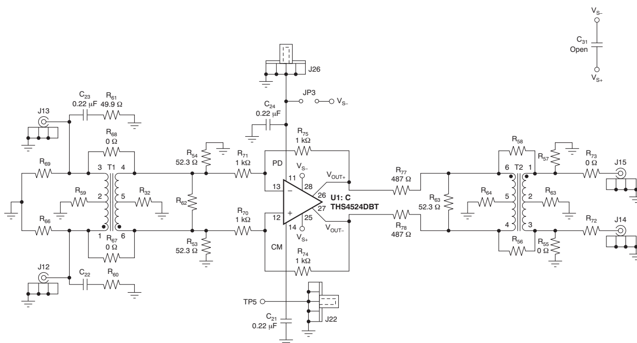
Figure 14. THS4524EVM: Schematic 3
