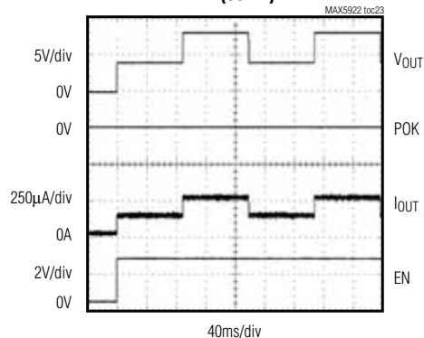
STARTUP WITH INVALID PD (33k \Omega )
