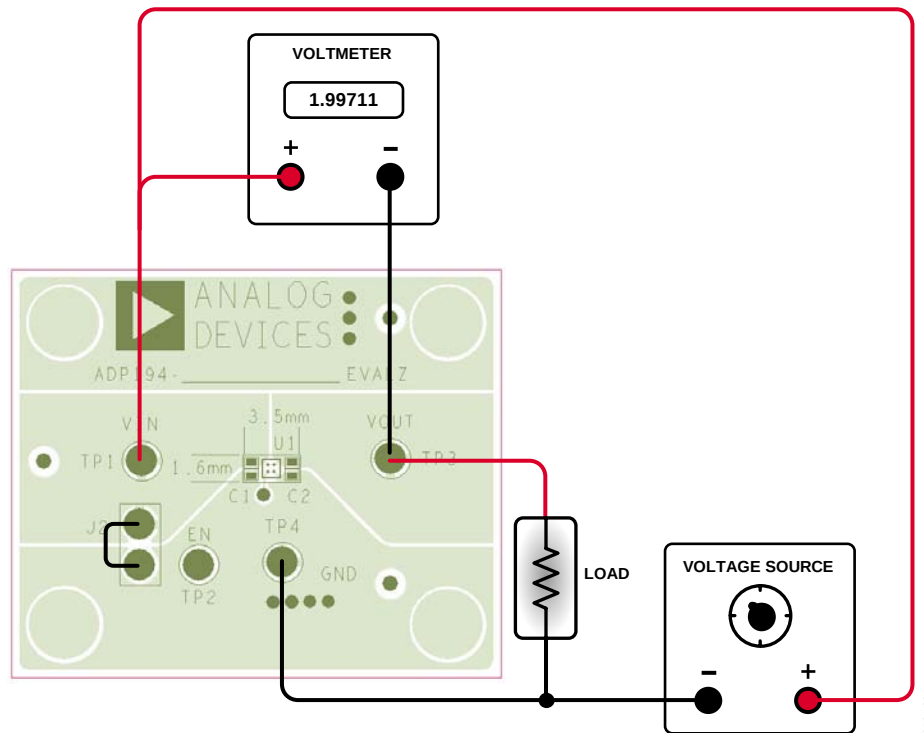
Figure 4. R_{DS_{ON}} Measurement
