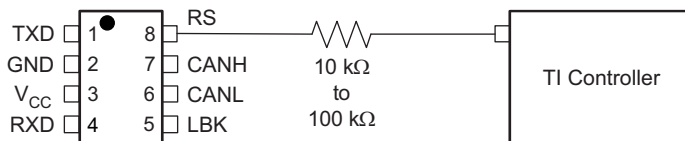
Figure 33. DSP Connection for Selecting Slope-Control or Standby Mode
