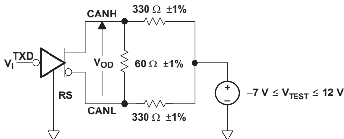
Figure 14. Driver V_{OD}
