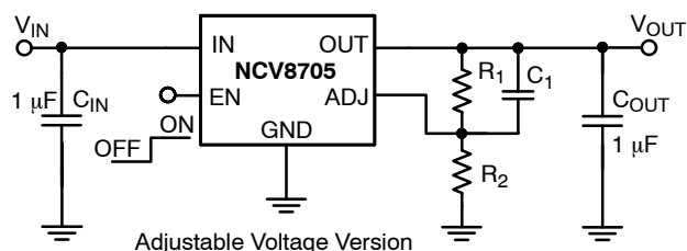
Figure 1. Typical Application Schematic
